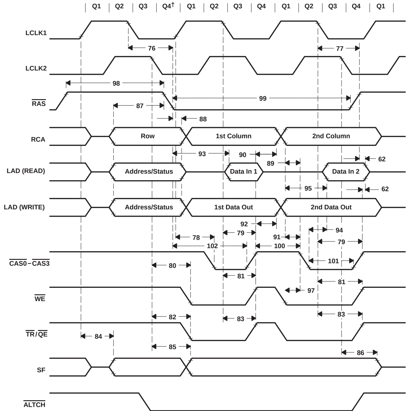
Figure 49. Local Bus: \overline{\text{RAS}} , \overline{\text{CAS0}}-\overline{\text{CAS3}} , \overline{\text{WE}} , \overline{\text{TR}}/\overline{\text{QE}} , and SF
