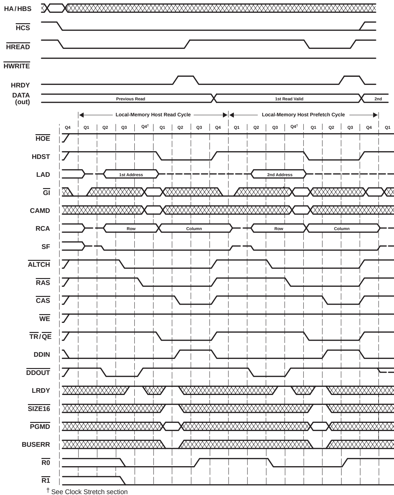
Figure 28. Back-to-Back Host Read Cycles With Implicit Addressing (HREAD as Strobe)
