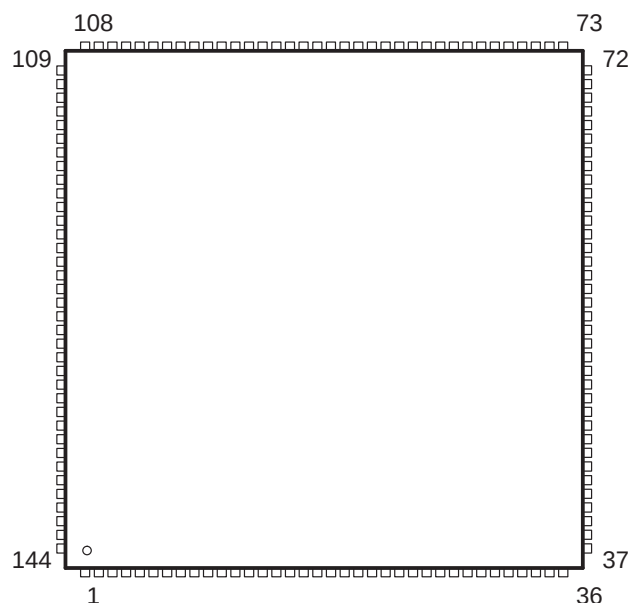
PCM PACKAGE (TOP VIEW)
