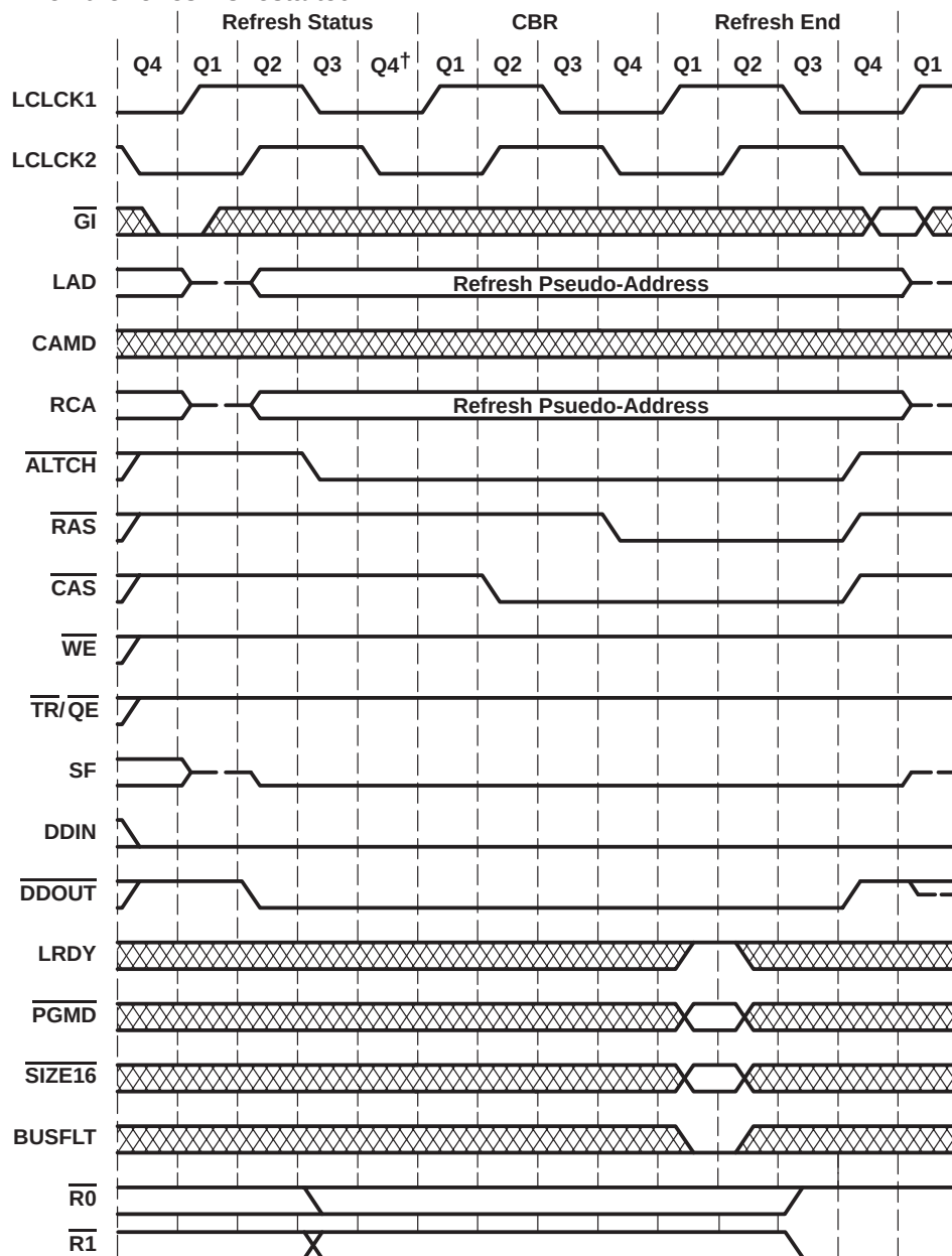
Figure 13. Refresh Cycle
