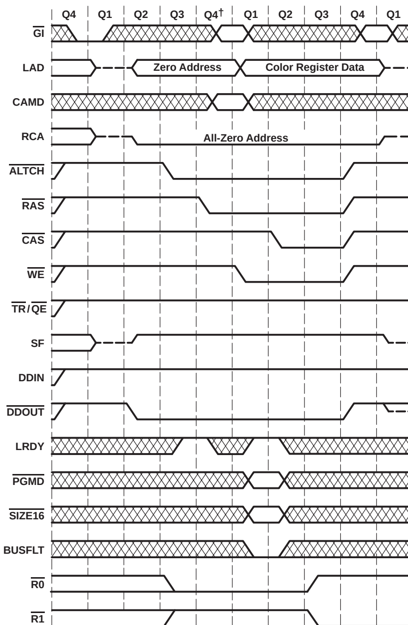
Figure 17. Load-Color-Latch Cycle
