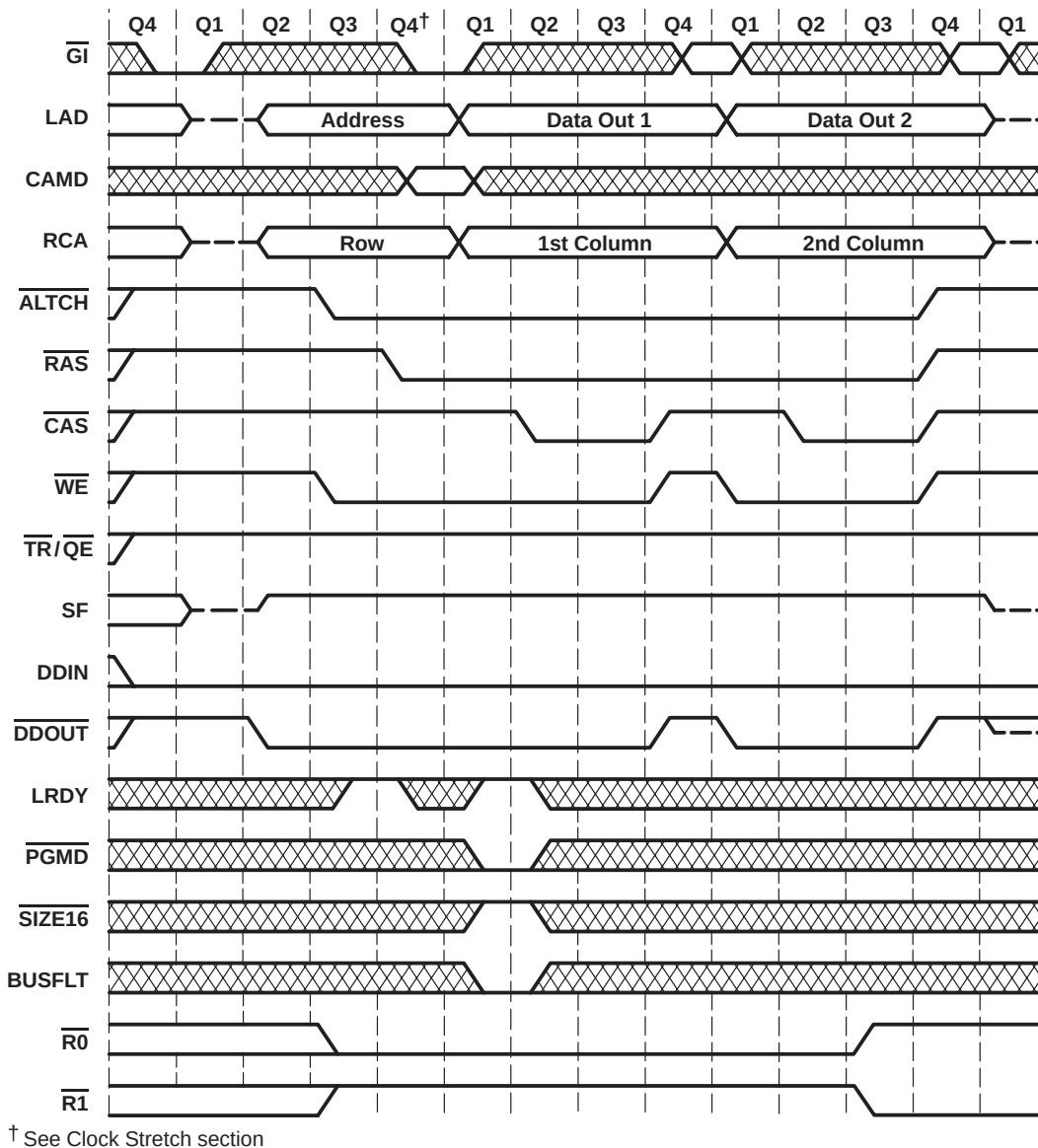
Figure 19. Block-Write Cycle (With Mask)
