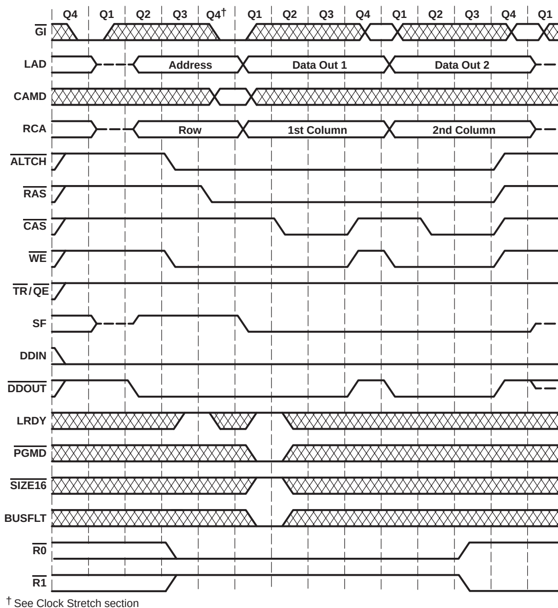
Figure 20. Write Cycle Using Mask
