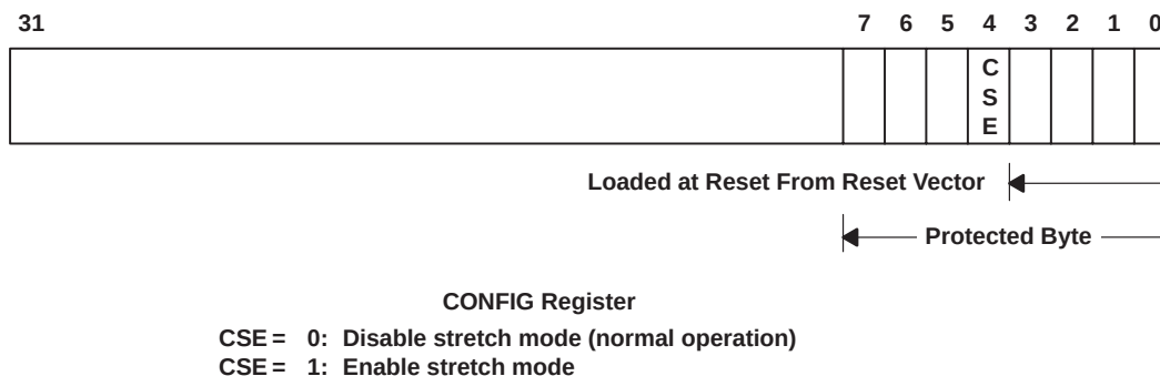
Figure 4. Stretch-Mode Enable
