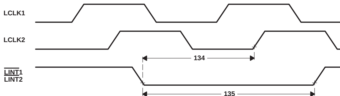
Figure 56. Interrupt: \overline{LINT1} and \overline{LINT2}
