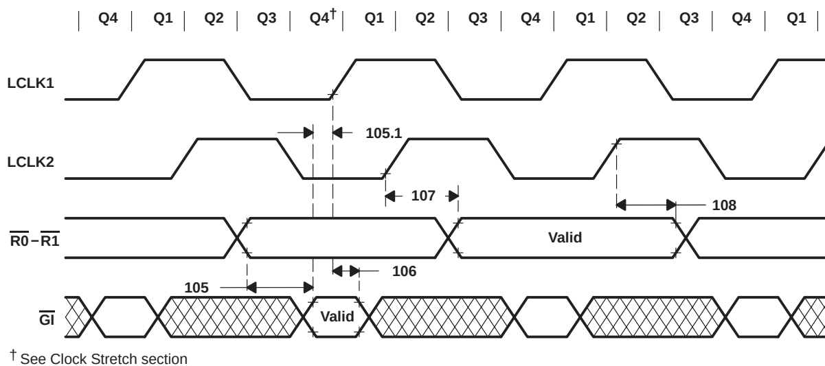
Figure 51. Multiprocessor Interface: \overline{\text{GI}} , \overline{\text{ALTCH}} , \overline{\text{RAS}} , \overline{\text{R0}} and \overline{\text{R1}}
