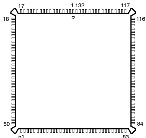
PQ PACKAGE (TOP VIEW)
