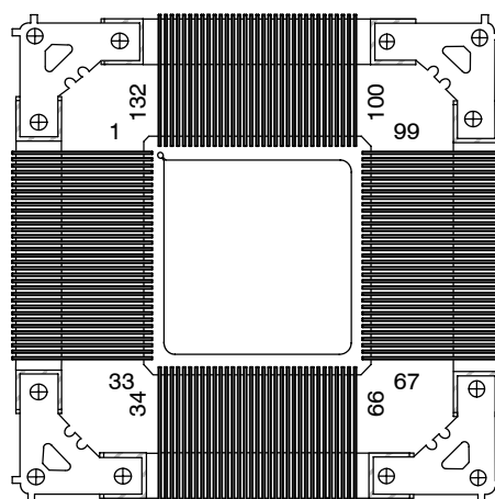
GFA PACKAGE (TOP VIEW)
