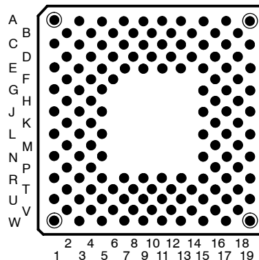
GFA PACKAGE (TOP VIEW)
