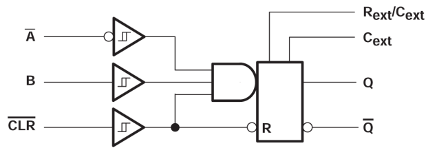
Logic Diagram, Each Multivibrator (Positive Logic)
