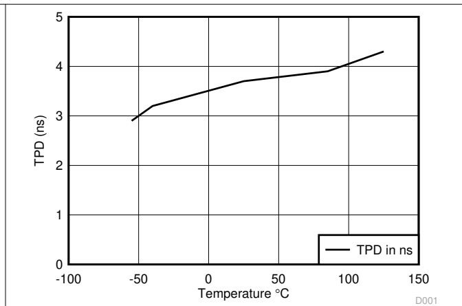
Figure 5-2. TPD vs Temperature
