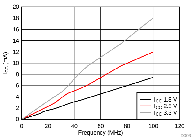
Figure 13. I_{CC} vs Frequency
