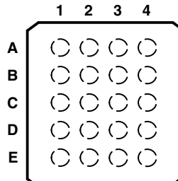
SN74LVTH573 . . . GQN OR ZQN PACKAGE (TOP VIEW)
