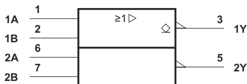
Figure 8-8. SNx5454B Logic Symbol
