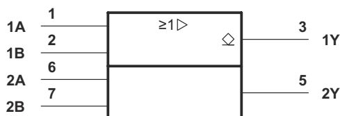
Figure 8-7. SNx5453B Logic Symbol
