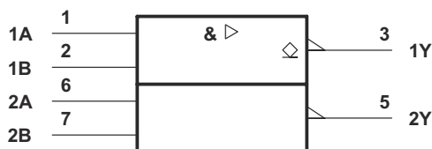
Figure 8-6. SNx5452B Logic Symbol
