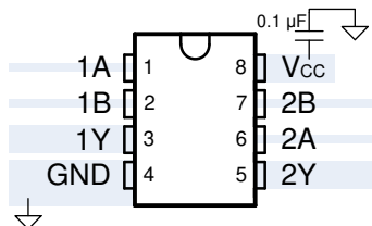
Figure 11-1. SN75451BD Layout
