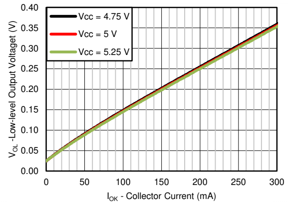
Figure 9-3. SN75451B Typical Low-Level Output Voltage vs Collector Current
