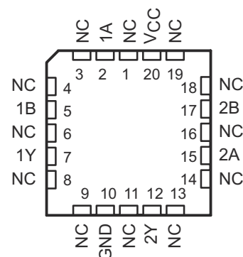
Figure 5-2. FK Package 20-Pin LCCC Top View
