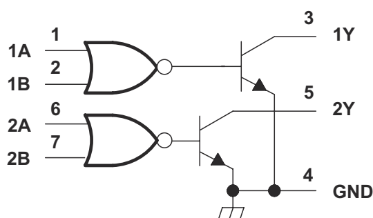
Figure 8-2. SNx5452B Logic Diagram (Positive Logic)
