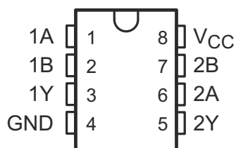
Figure 5-1. JG, D, P, or PS Package 8-Pin CDIP, SOIC, PDIP, or SO Top View
