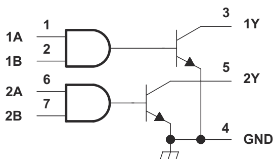
Figure 8-1. SNx5451B Logic Diagram (Positive Logic)
