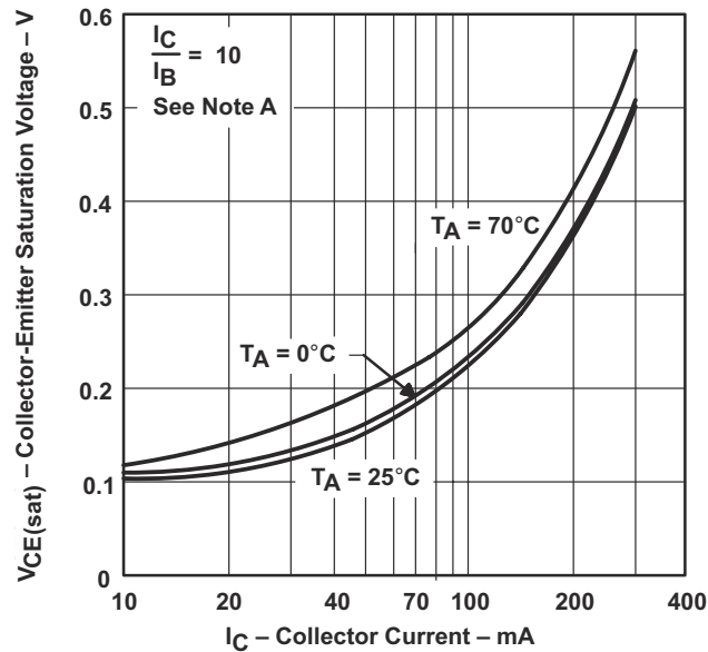
Figure 6-1. Transistor Collector-Emitter Saturation Voltage vs Collector Current
