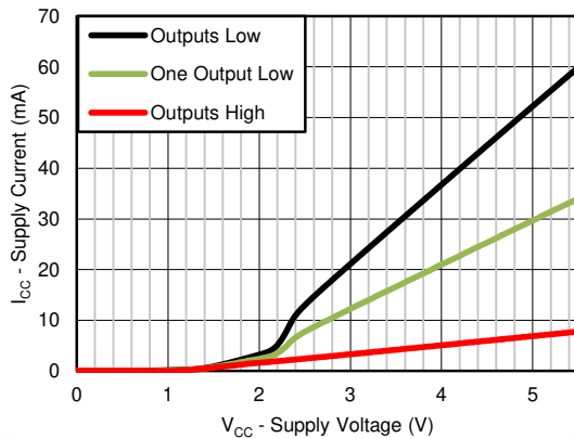
Figure 9-2. SN75451B Typical Supply Current vs Supply Voltage
