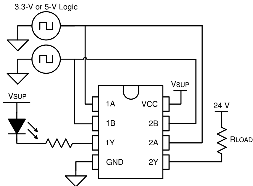
Figure 9-1. SN75451B Driving an LED and a High Voltage Peripheral
