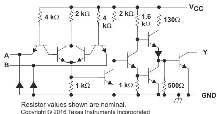
Figure 8-12. SNx5454B Schematic (Each Driver)
