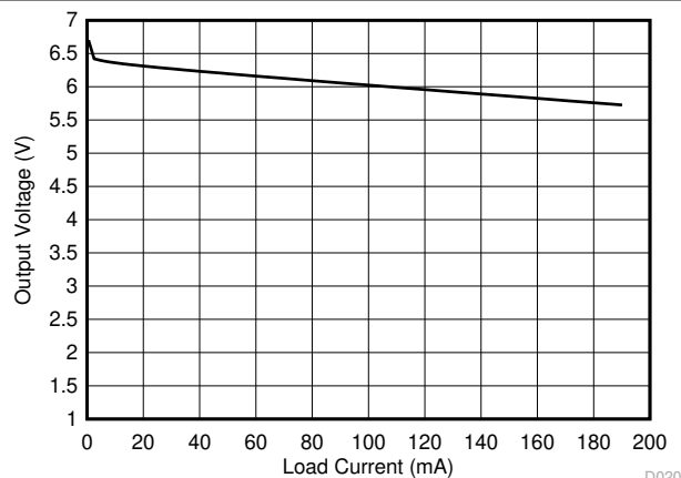
Figure 6-23. Output Voltage vs Load Current
