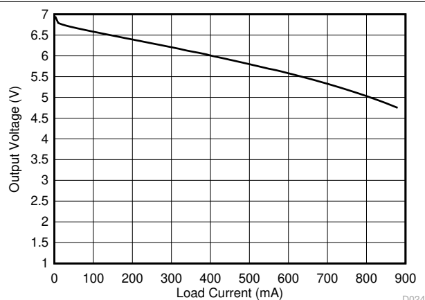
Figure 6-25. Output Voltage vs Load Current
