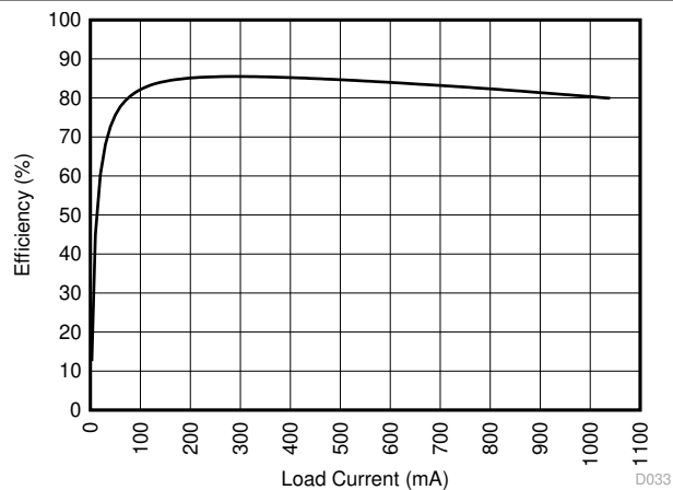
Figure 6-8. Efficiency vs Load Current
