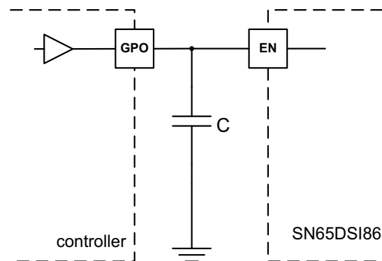
Figure 7. EN Input from Active Controller
