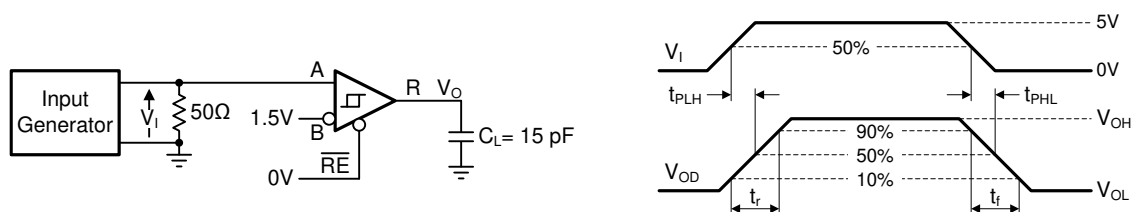
Figure 6-6. Measurement of Receiver Output Rise and Fall Times and Propagation Delays
