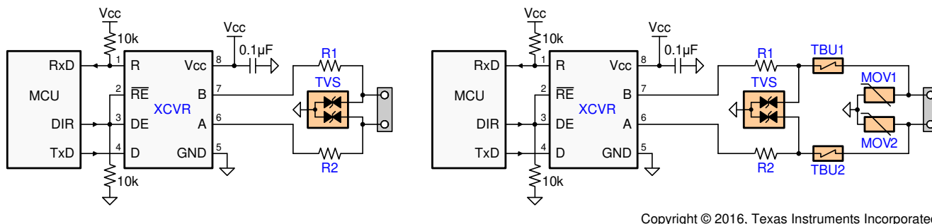
Figure 8-8. Transient Protections Against ESD, EFT, and Surge Transients
