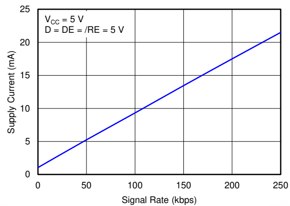
Figure 5-3. Supply Current vs Signaling Rate
