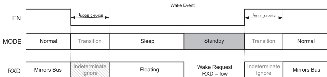
Figure 7-3. Mode Transitions
