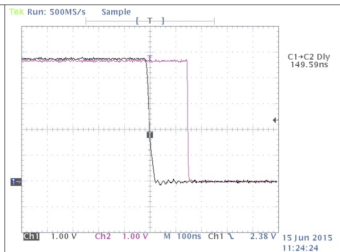
Figure 21. tLoop Delay Waveform Recessive to Dominant
