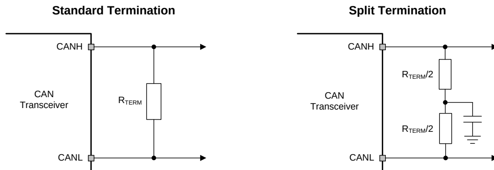
Figure 18. CAN Termination Scheme
