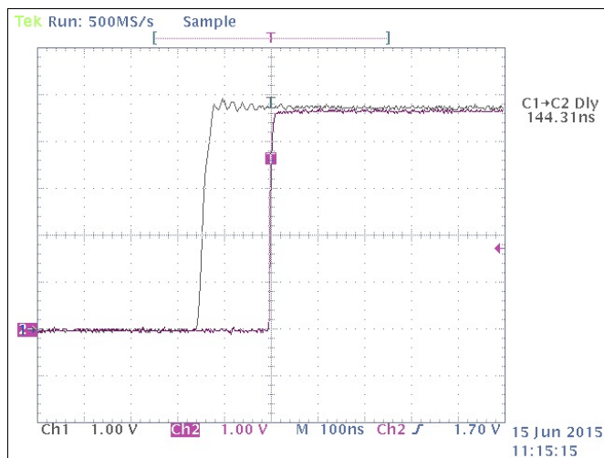
Figure 20. tLoop Delay Waveform Dominant to Recessive
