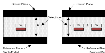
Figure 52. Stripline Topology
