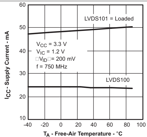
Figure 2. Supply Current vs Free-Air Temperature
