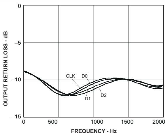
Figure 6-19. Output Return Loss
