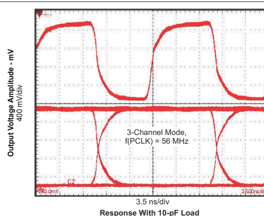
Figure 6-17. XGA 3-channel Output Waveform on the SN65LVDS302 when driven by the SN65LVDS301
