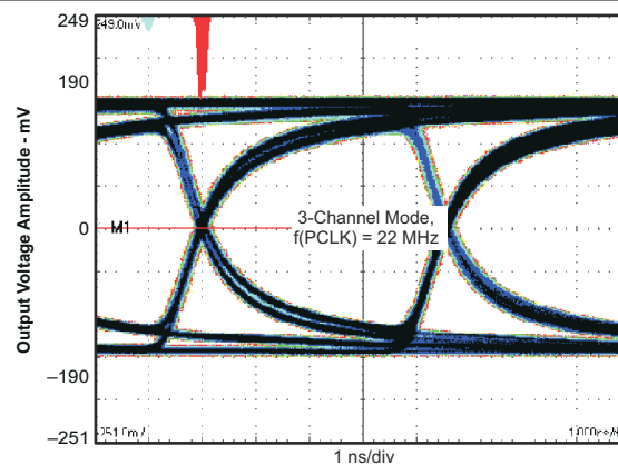
Figure 6-15. VGA 3-channel Output Waveform
