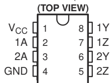
SN65LVDS9638DGK (Marked as AXG)
