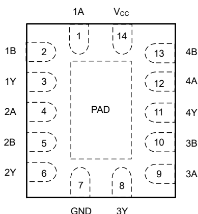
Figure 4-1. SN74AC09 BQA Package (Top View)
