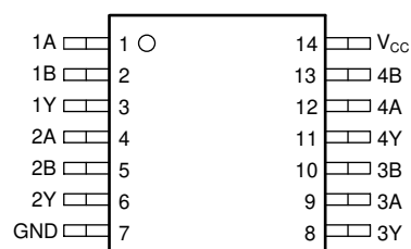
Figure 4-2. SN74AC09, PW Package (Top View)
