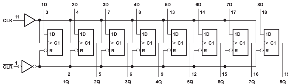
Simplified Schematics
