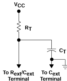
Figure 7-1. Timing-Component Connections
