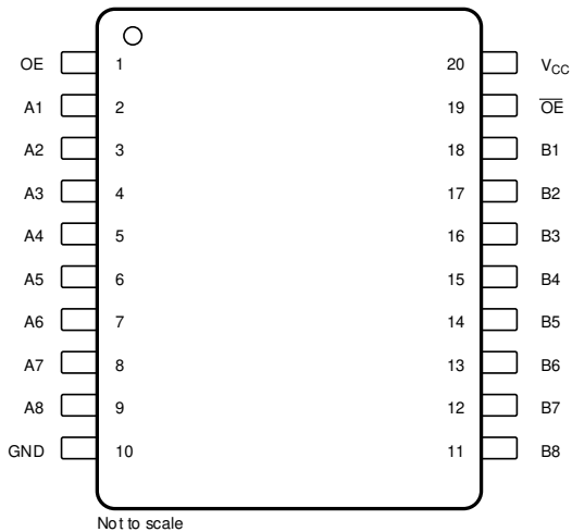
Figure 4-1. DBQ, DGV, or PW Package, SOP 20-Pins (Top View)
