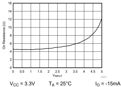
Figure 5-1. Typical r_{on} vs V_I
