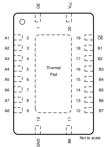
Figure 4-2. RGY Package, VQFN 20-Pins (Top View)
