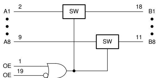
Figure 7-1. Logic Diagram (Positive Logic)
