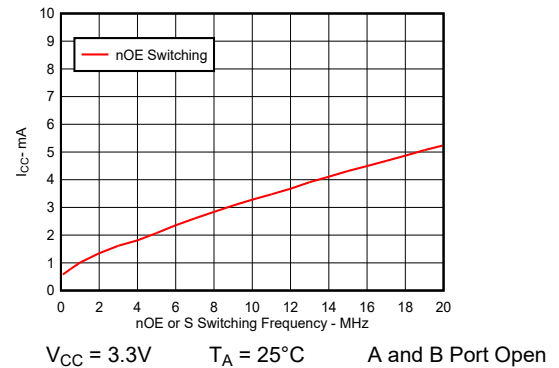
Figure 5-2. Typical I_{CC} vs OE or \overline{OE} Switching Frequency
