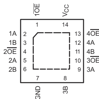
Figure 4-2. BQA Package 14-Pin WQFN Top View
