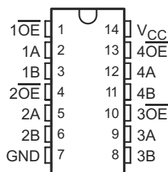
Figure 4-1. PW, DYY Package 14-Pin TSSOP, SOT Top View
