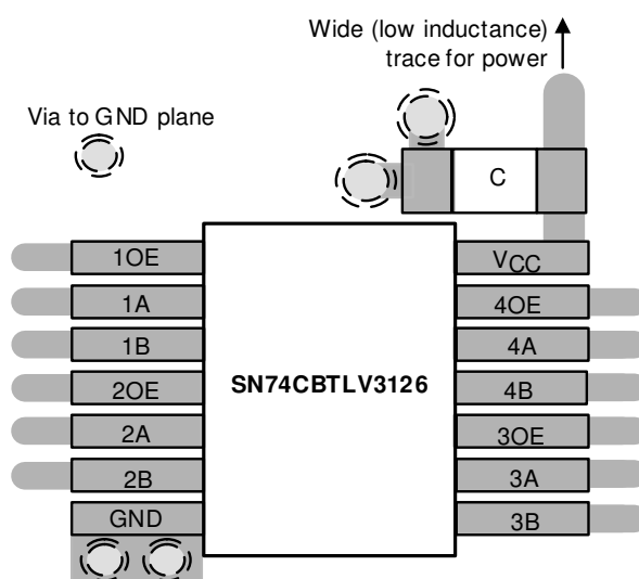
Figure 8-4. Example Layout
