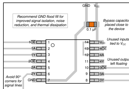
Figure 8-3. Example layout for the SN74HCS125-Q1
