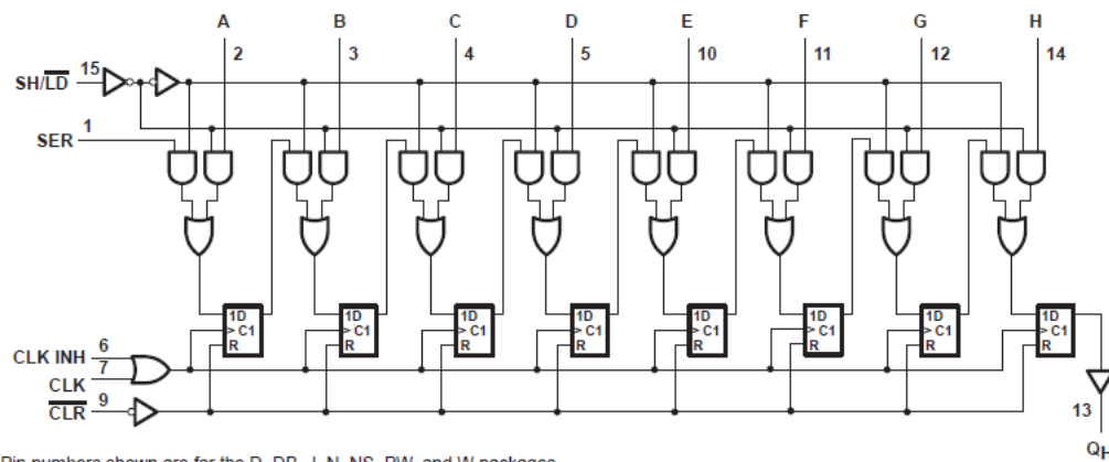
Pin numbers shown are for the D, DB, J, N, NS, PW, and W packages.
