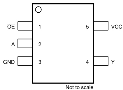
Figure 5-1. DCK or DBV Package, 5-Pin SC70 or SOT-23 (Top View)
