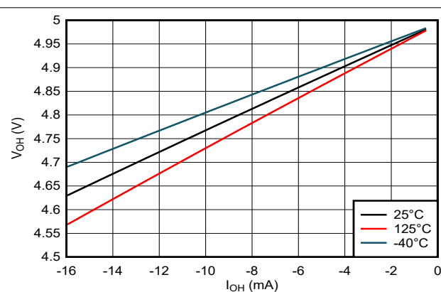
Figure 6-2. Output Voltage vs Current in HIGH State; 5V Supply
