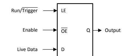
Figure 8-1. Typical Application Schematic
