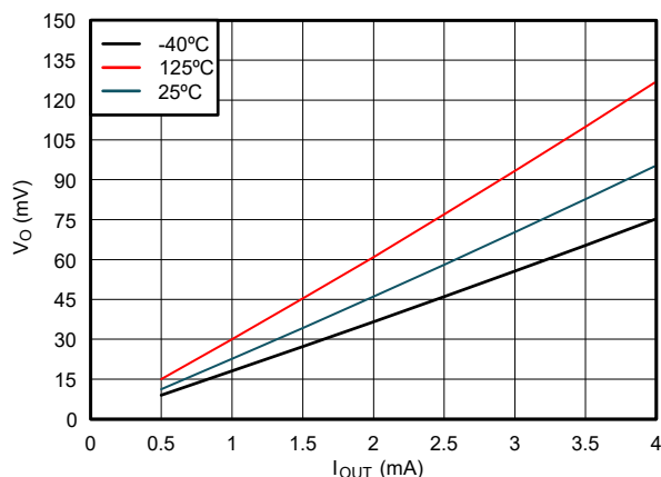
Figure 5-5. Output Voltage vs Current in LOW State; 1.65V Supply
