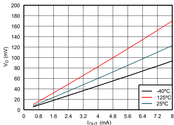
Figure 5-4. Output Voltage vs Current in LOW State; 2.3V Supply
