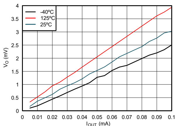
Figure 5-6. Output Voltage vs Current in LOW State; 1.38V Supply
