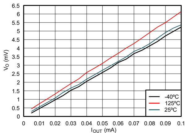
Figure 5-7. Output Voltage vs Current in LOW State; 1.1V Supply
