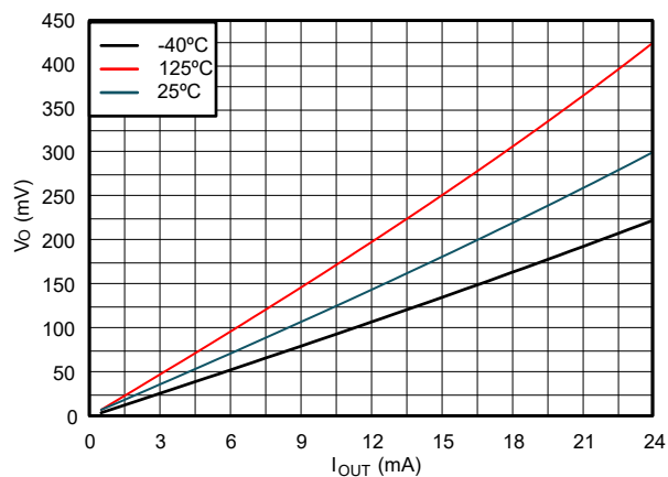
Figure 5-3. Output Voltage vs Current in LOW State; 3V Supply
