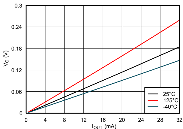
Figure 5-5. Output Voltage vs Current in LOW State; 4.5V Supply
