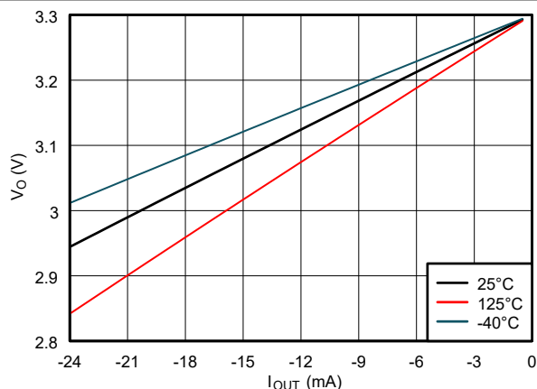
Figure 5-6. Output Voltage vs Current in HIGH State; 3.3V Supply
