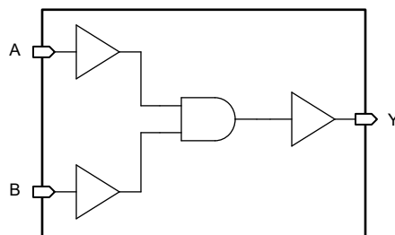
Figure 7-1. Logic Diagram (Positive Side)
