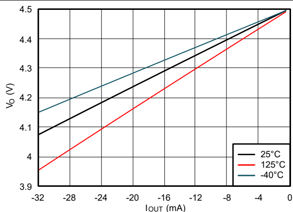
Figure 5-4. Output Voltage vs Current in HIGH State; 4.5V Supply
