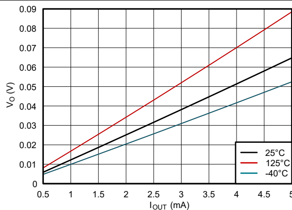
Figure 5-11. Output Voltage vs Current in LOW State; 1.8V Supply
