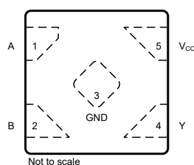
Figure 4-2. DTX Package 5-PIN X2SON Top View
