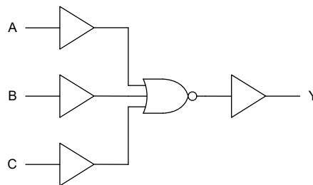
Figure 7-1. Logic Diagram (Positive Logic) for SN74LVC1G27B-Q1
