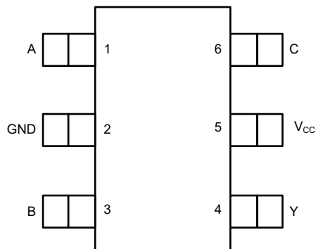
Figure 4-1. DCK or DBV Package, 6-Pin SC-70 or SOT-23 (Top View)
