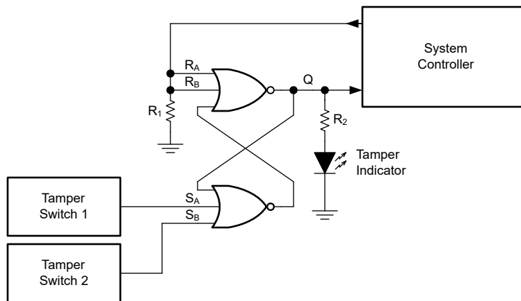
Figure 8-1. Application Block Diagram
