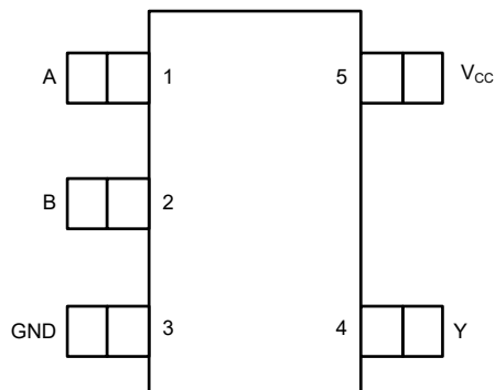
Figure 4-1. DBV or DCK or DRL Package, 5-Pin SOT-23 or SOT-SC70SOT (Top View)
