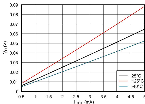
Figure 5-6. Output Voltage vs Current in LOW State; 1.8V Supply
