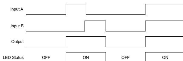
Figure 8-2. Application timing diagram
