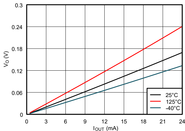
Figure 5-4. Output Voltage vs Current in LOW State; 3.3V Supply
