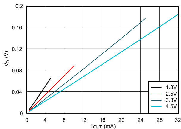
Figure 5-2. Output Voltage vs Current in LOW State
