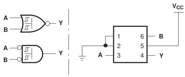
Figure 7-5. 2-Input NOR Gate
