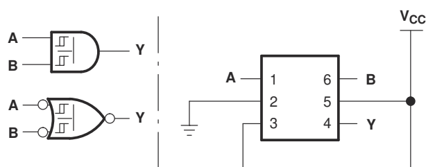
Figure 7-2. 2-Input AND Gate
