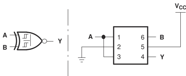
Figure 7-6. 2-Input XNOR Gate
