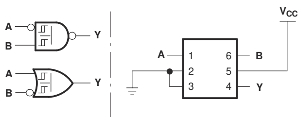
Figure 7-3. 2-Input NAND Gate With Inverted A Input
