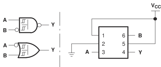
Figure 7-4. 2-Input NAND Gate With Inverted B Input
