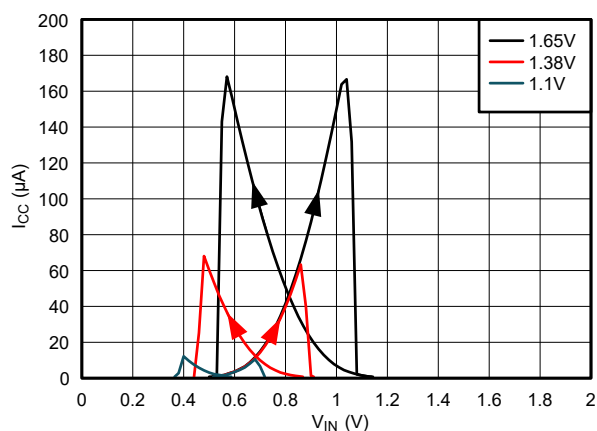
Figure 5-2. Supply Current Across Input Voltage 1.1V to 1.65V Supply
