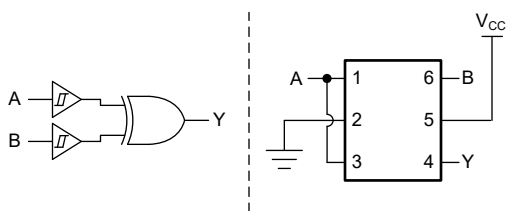
Figure 7-6. 2-Input XOR Gate
