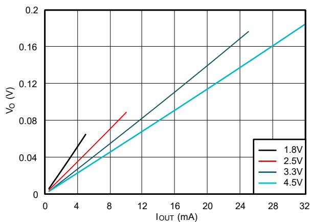
Figure 5-5. Output Voltage vs Current in LOW State
