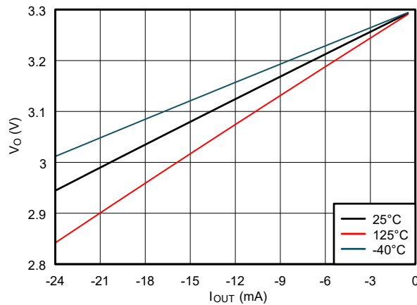
Figure 5-8. Output Voltage vs Current in HIGH State; 3.3V Supply
