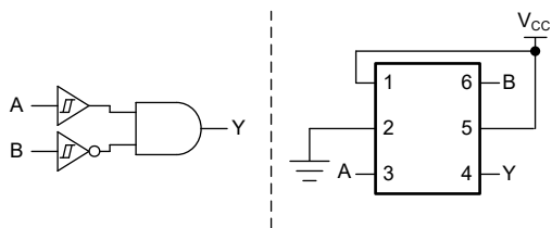
Figure 7-4. 2-Input AND Gate With Inverted B Input
