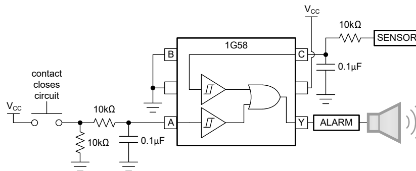
Figure 8-1. Typical Application Diagram
