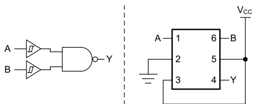
Figure 7-2. 2-Input NAND Gate
