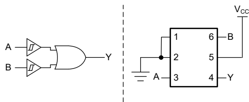
Figure 7-5. 2-Input OR Gate
