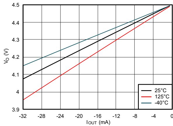
Figure 5-6. Output Voltage vs Current in HIGH State; 4.5V Supply
