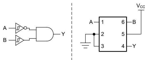
Figure 7-3. 2-Input AND Gate With Inverted A Input
