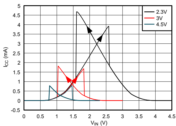
Figure 5-3. Supply Current Across Input Voltage 2.3V to 4.5V Supply
