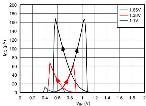
Figure 5-2. Supply Current Across Input Voltage 1.1V to 1.65V Supply
