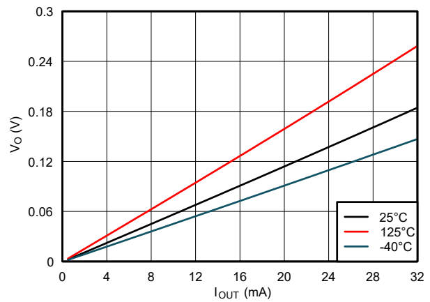
Figure 5-7. Output Voltage vs Current in LOW State; 4.5V Supply
