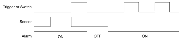
Figure 8-2. Trigger, Sensor and Alarm Timing Diagram
