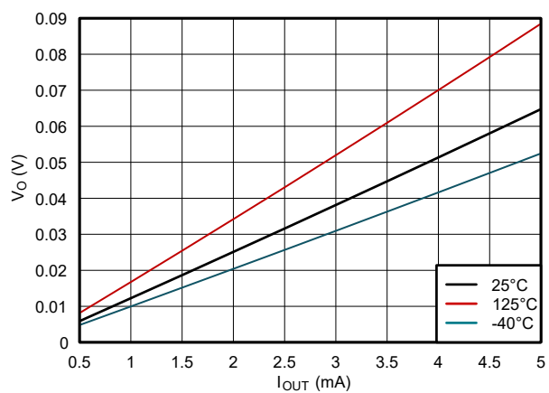
Figure 5-13. Output Voltage vs Current in LOW State; 1.8V Supply
