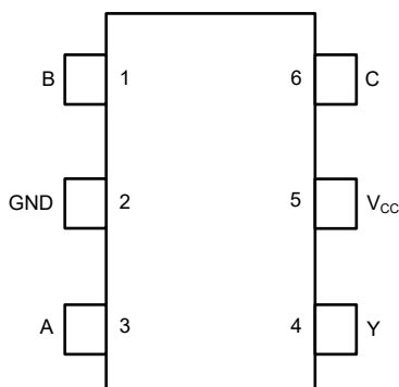
Figure 4-1. DCK, DBV Package6-Pin SC70, SOT-23Top View
