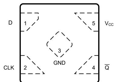
Figure 4-2. DTX Package, 5-Pin X2SON (Top View)
