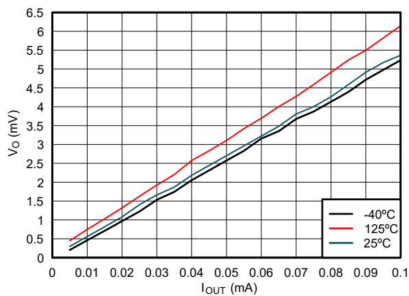
Figure 5-9. Output Voltage vs Current in LOW State; 1.1V Supply
