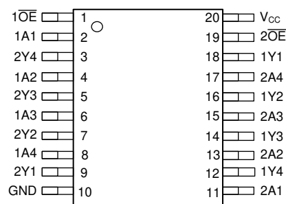
Figure 4-2. SN74LVC244B PW Package (Top View)
