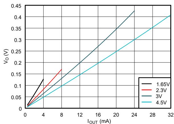
Figure 5-3. Output Voltage vs Current in LOW State
