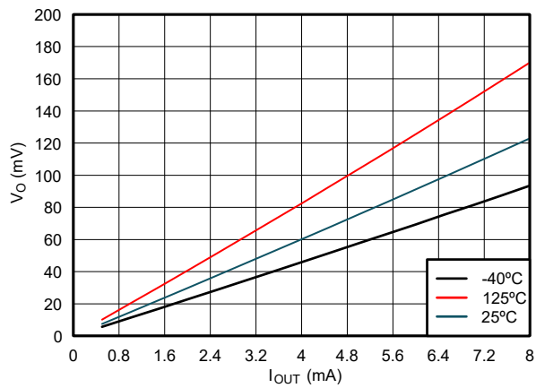
Figure 5-6. Output Voltage vs Current in LOW State; 2.3V Supply
