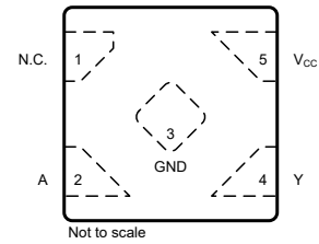
Figure 4-2. DPW Package, 5-Pin X2SON (Top View)
