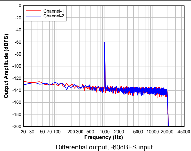
Figure 5-11. DAC FFT
