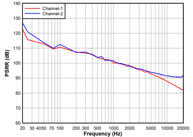
Figure 5-13. DAC PSRR vs Frequency
