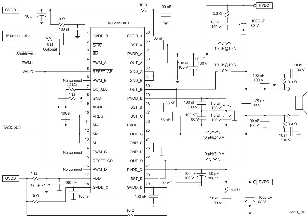
Figure 18. Typical Non-Differential (1N) PBT Application (For Reference Only, component values and connection will change.)
