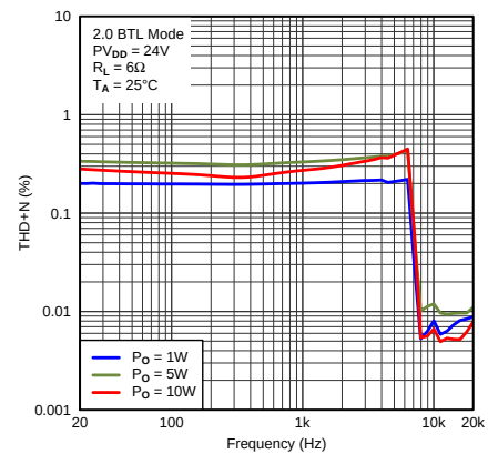
Figure 14. THD+N vs Frequency
