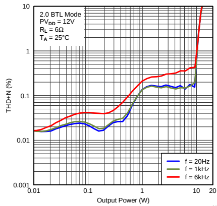
Figure 17. THD+N vs Output Power
