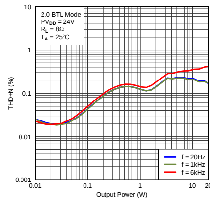
Figure 22. THD+N vs Output Power
