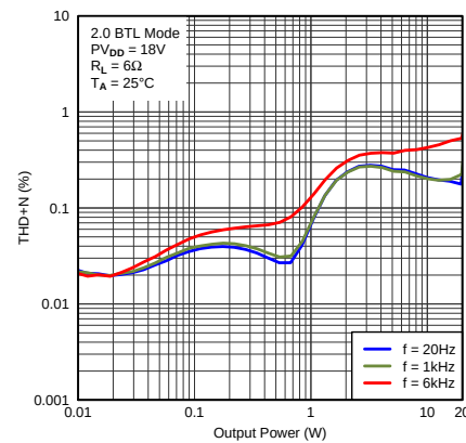
Figure 20. THD+N vs Output Power
