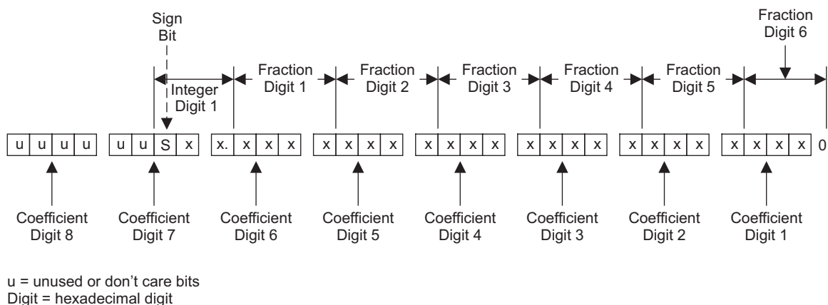
Figure 66. Alignment of 3.23 Coefficient in 32-Bit I²C Word
