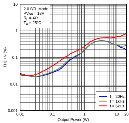
Figure 21. THD+N vs Output Power
