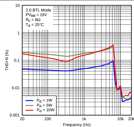
Figure 10. THD+N vs Frequency
