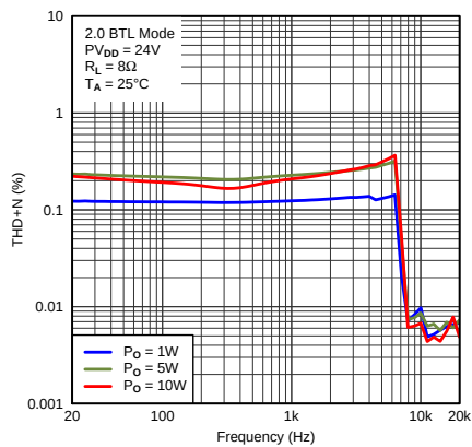
Figure 13. THD+N vs Frequency
