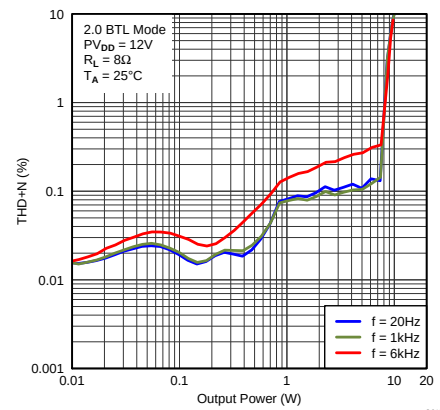
Figure 16. THD+N vs Output Power
