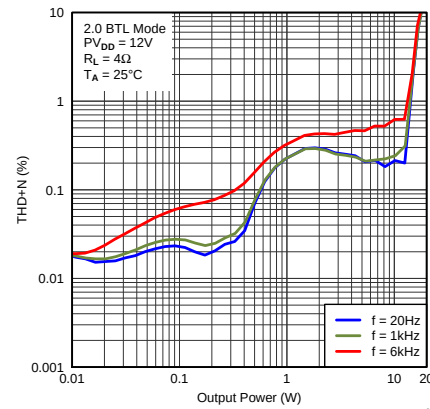
Figure 18. THD+N vs Output Power
