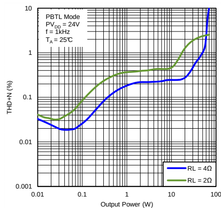
Figure 36. Total Harmonic Distortion + Noise vs Output Power (PBTL Mode)
