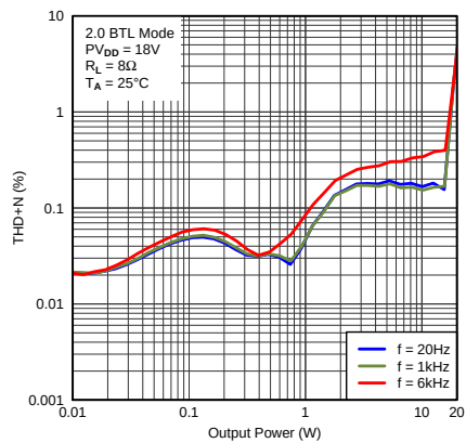
Figure 19. THD+N vs Output Power
