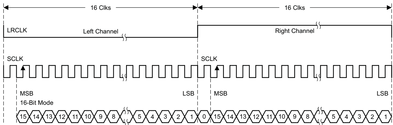
Figure 57. I 2 S 32-f s Format
