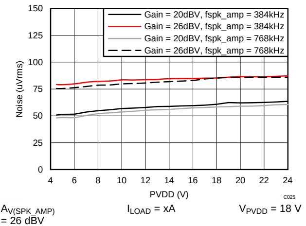
Figure 51. Idle Channel Noise vs VPD – PBTL
