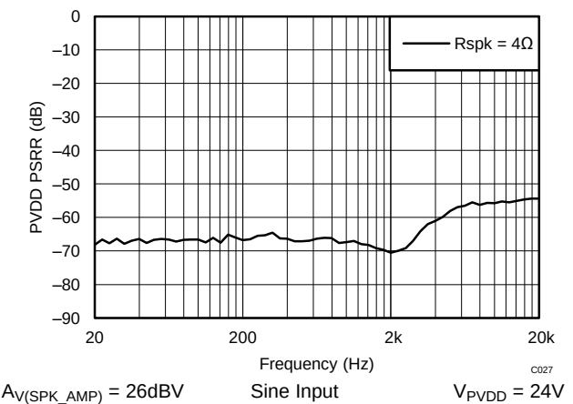
Figure 53. VPD PSRR vs Frequency – PBTL
