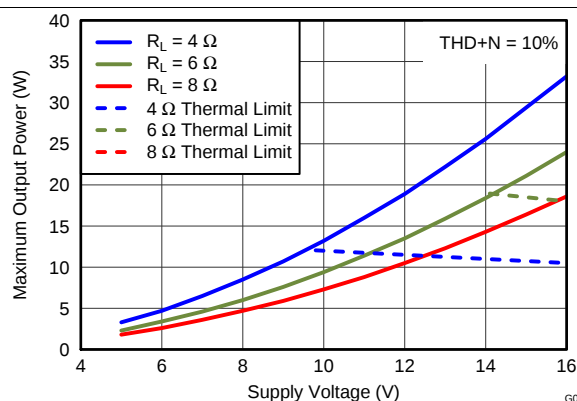
Thermal Limits are referenced to TAS5760xxEVM Rev D Figure 14. Output Power vs PVDD
