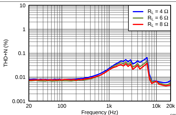
PVDD = 12 V, P_{\text{OSPK}} = 1 \text{ W} Figure 16. THD+N vs Frequency
