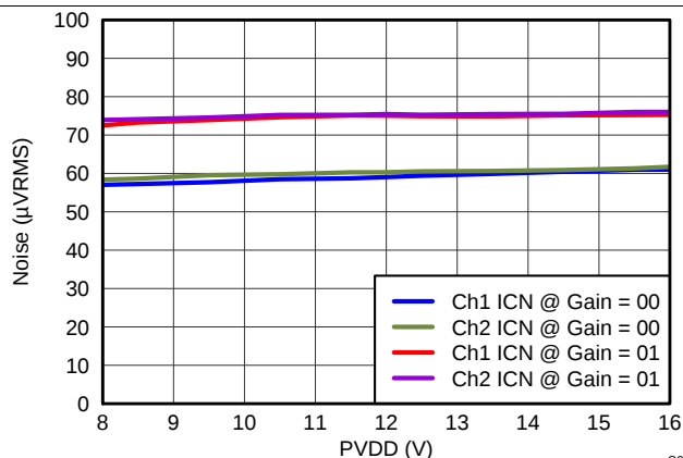
Figure 17. Idle Channel Noise vs PVDD
