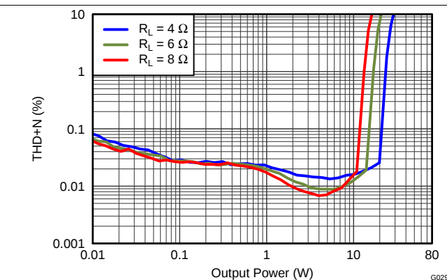
PVDD = 12 V, Both Channels Driven Figure 6. THD+N vs Output Power
