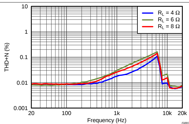
PVDD = 12 V, P_{\text{OSPK}} = 1 \text{ W} Figure 15. THD+N vs Frequency
