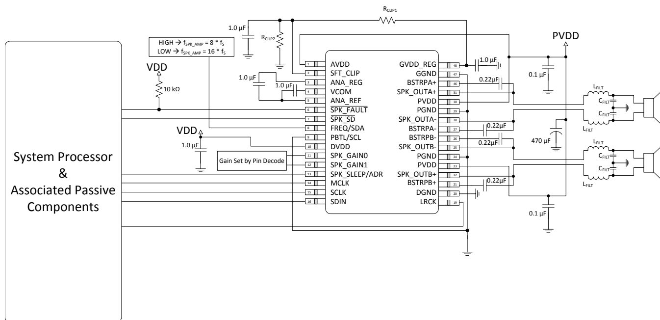
Figure 62. Stereo BTL using Hardware Control, 32-Pin DAP Package Option
