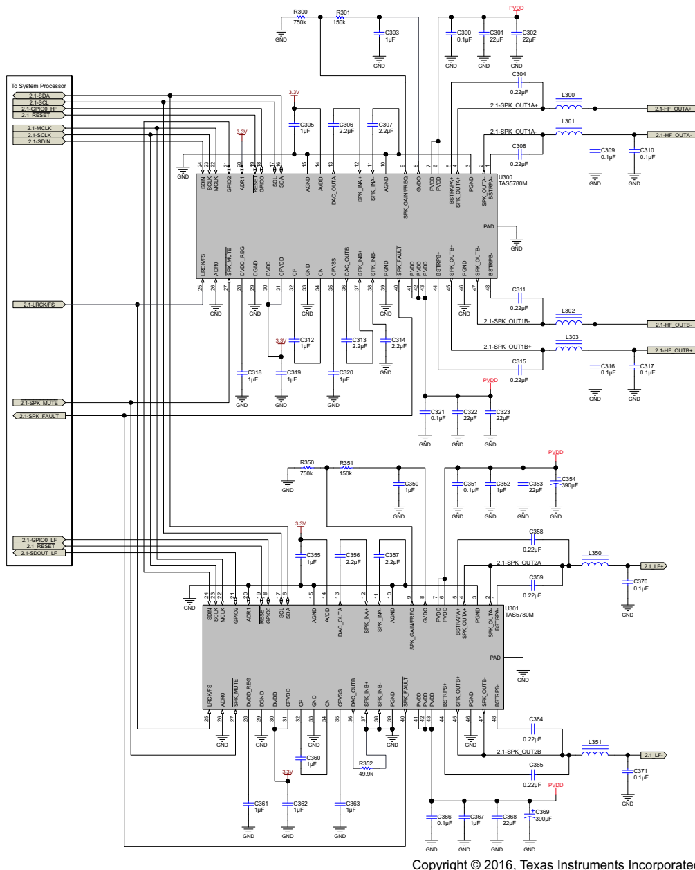
Figure 86. 2.1 (Stereo BTL + External Mono Amplifier) Application Schematic
