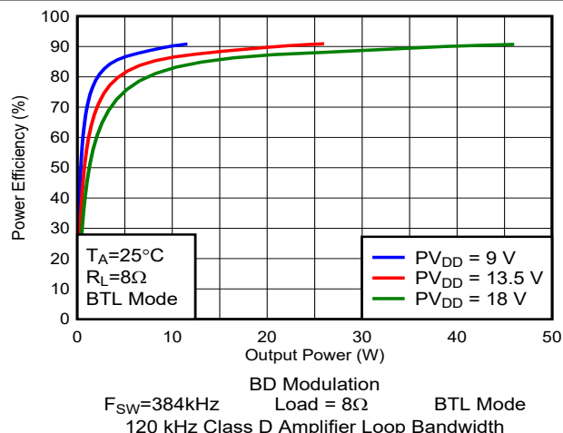
Figure 5-66. Efficiency vs Output Power
