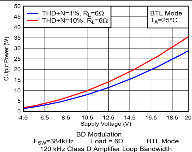
Figure 5-56. Output Power vs Supply Voltage
