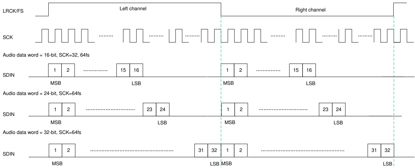
Figure 6-2. Left Justified Audio Data Format
