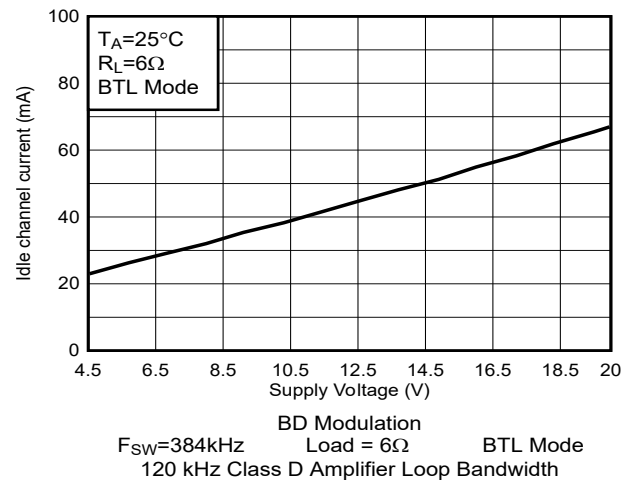
Figure 5-64. PVDD Idle Current vs PVDD Voltage
