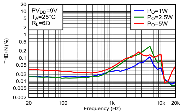
Figure 5-4. THD+N vs Frequency
