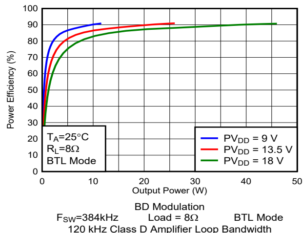
Figure 5-67. Efficiency vs Output Power
