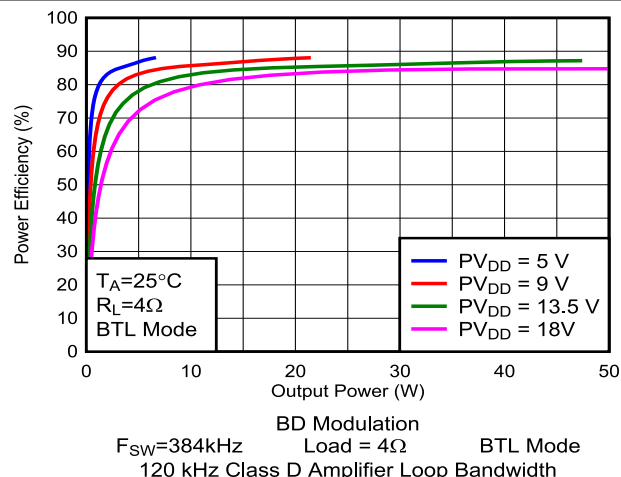
Figure 5-65. Efficiency vs Output Power
