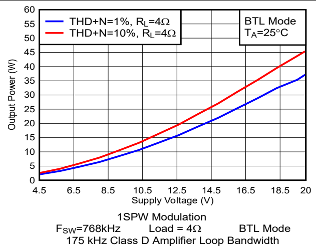
Figure 5-18. Output Power vs Supply Voltage
