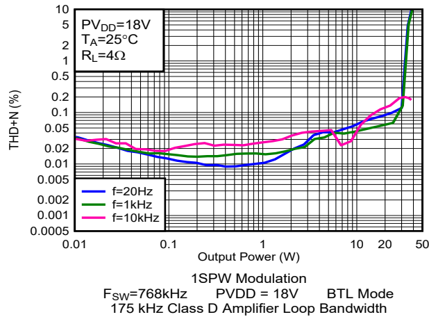
Figure 5-13. THD+N vs Output Power
