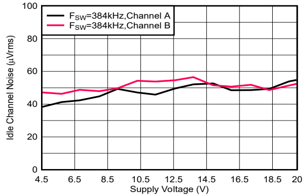
Figure 5-59. Idle Channel Noise vs Supply Voltage
