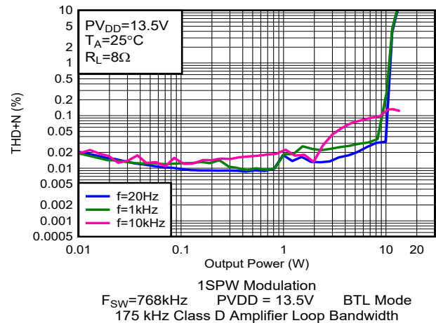
Figure 5-16. THD+N vs Output Power
