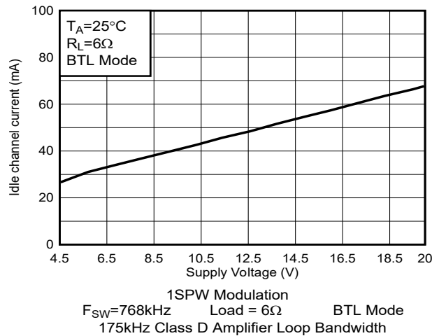
Figure 5-29. PVDD Idle Current vs PVDD Voltage
