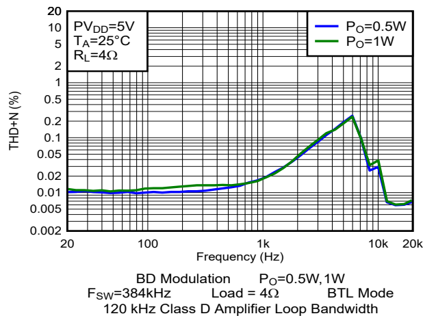
Figure 5-33. THD+N vs Frequency
