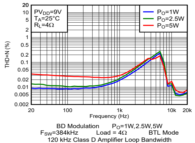
Figure 5-34. THD+N vs Frequency
