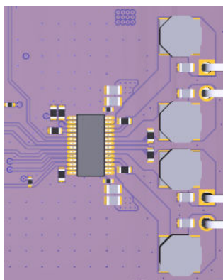
Top Layer 3D view
