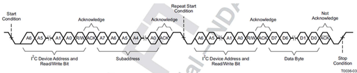
Figure 6-14. Random Read Transfer
