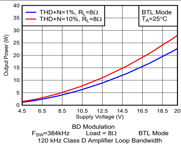
Figure 5-57. Output Power vs Supply Voltage
