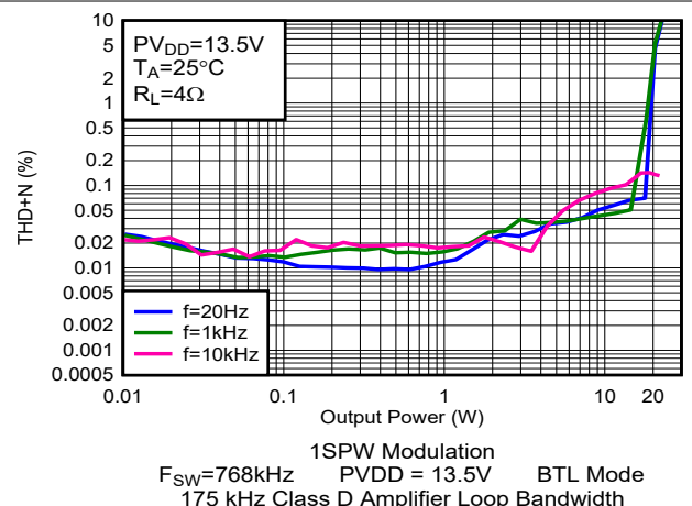
Figure 5-12. THD+N vs Output Power
