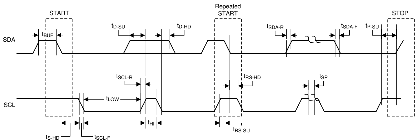
Figure 6-8. I²C Communication Timing - Target
