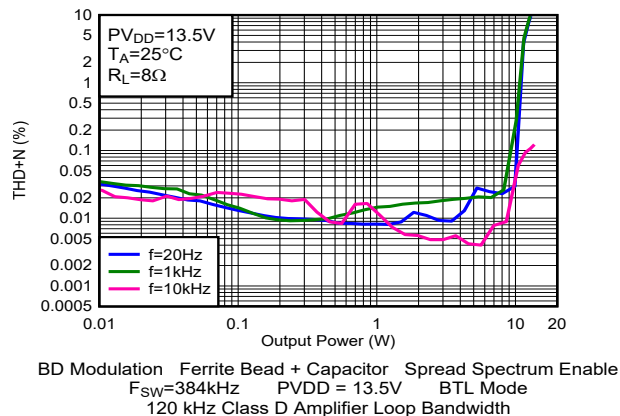
Figure 5-54. THD+N vs Output Power
