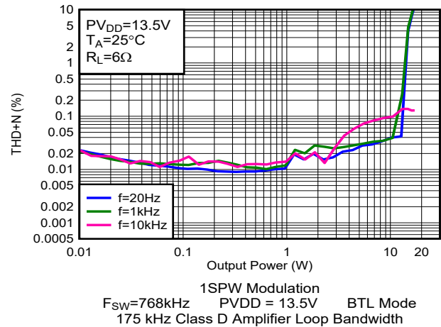
Figure 5-14. THD+N vs Output Power
