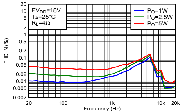
Figure 5-2. THD+N vs Frequency
