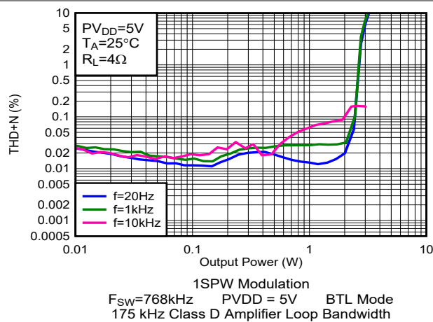
Figure 5-11. THD+N vs Output Power
