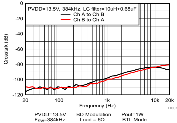
Figure 5-25. Crosstalk
