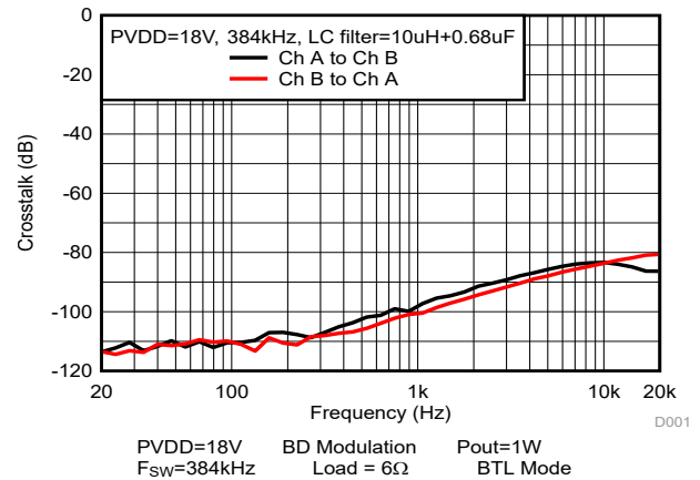
Figure 5-62. Crosstalk
