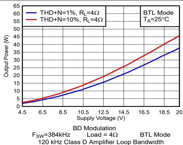
Figure 5-55. Output Power vs Supply Voltage
