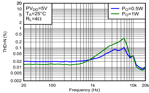
Figure 5-1. THD+N vs Frequency
