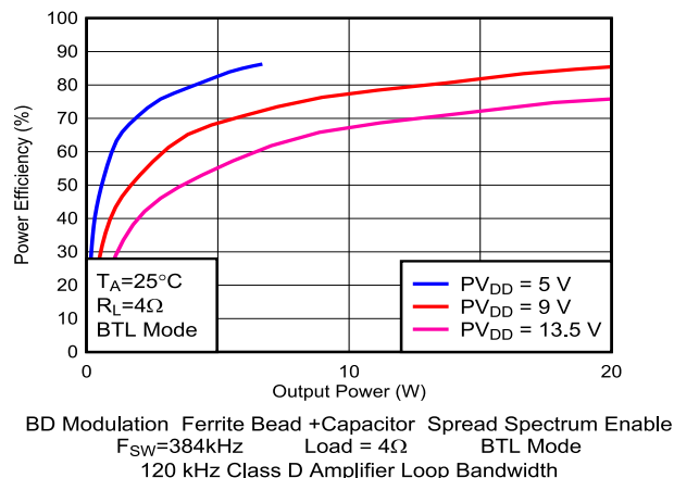
Figure 5-68. Efficiency vs Output Power (with FB)
