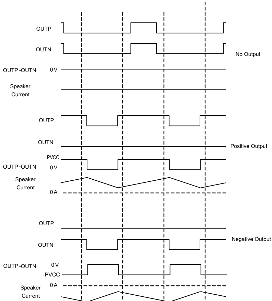
Figure 6-11. 1SPW Mode Modulation
