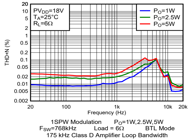
Figure 5-8. THD+N vs Frequency
