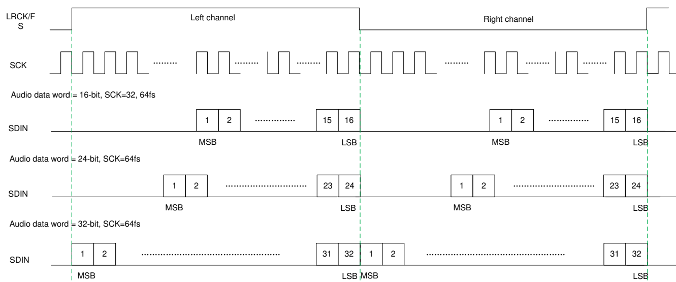
Figure 6-3. I²S Audio Data Format
