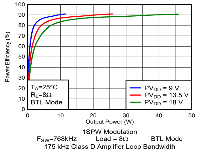
Figure 5-32. Efficiency vs Output Power
