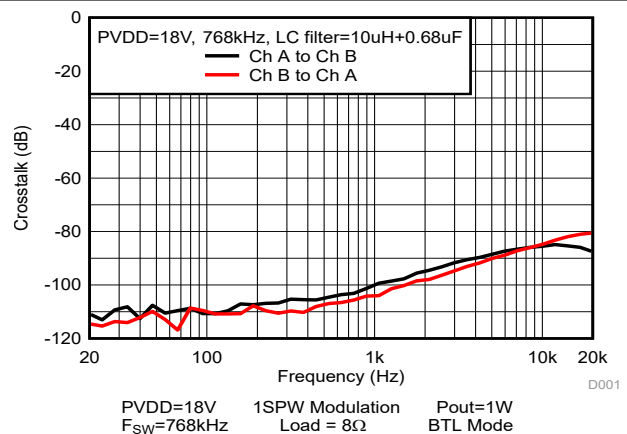
Figure 5-28. Crosstalk
