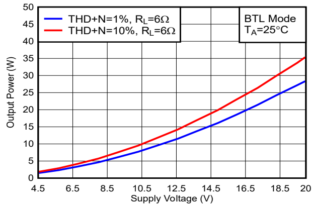
Figure 5-19. Output Power vs Supply Voltage
