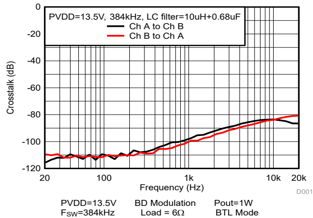
Figure 5-61. Crosstalk
