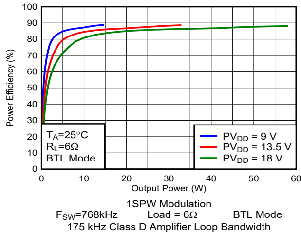
Figure 5-31. Efficiency vs Output Power
