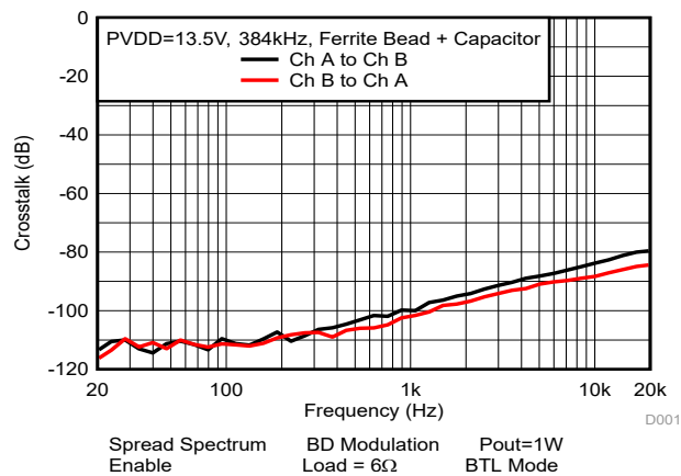
Figure 5-63. Crosstalk
