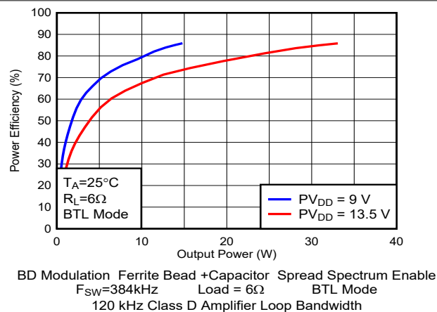
Figure 5-69. Efficiency vs Output Power
