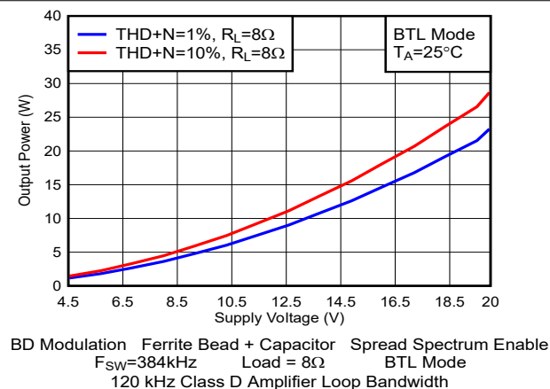
Figure 5-58. Output Power vs Supply Voltage
