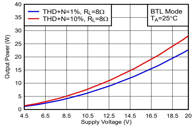
Figure 5-20. Output Power vs Supply Voltage
