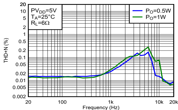
Figure 5-3. THD+N vs Frequency
