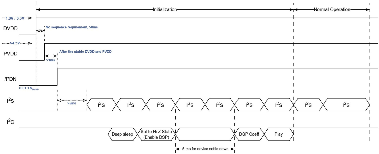
Figure 6-16. Startup sequence
