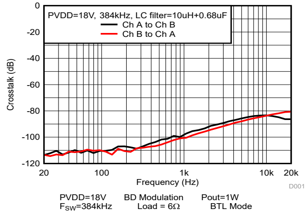
Figure 5-26. Crosstalk
