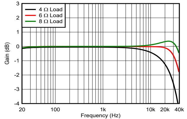
Figure 5-60. Gain vs Frequency
