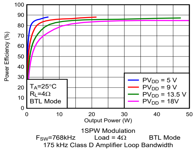
Figure 5-30. Efficiency vs Output Power
