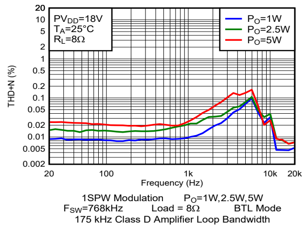
Figure 5-10. THD+N vs Frequency
