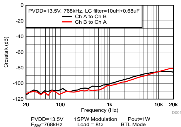
Figure 5-27. Crosstalk
