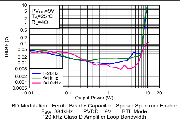
Figure 5-52. THD+N vs Output Power
