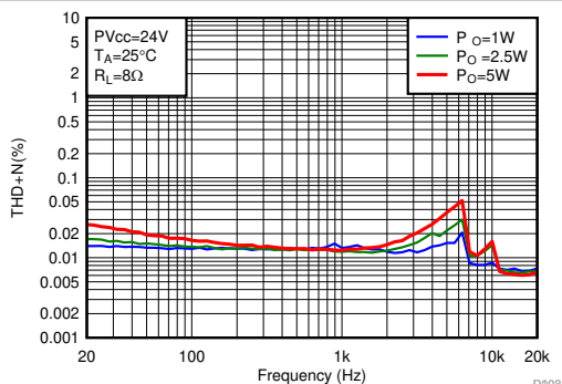
Figure 6-9. THD+N vs Frequency-BTL
