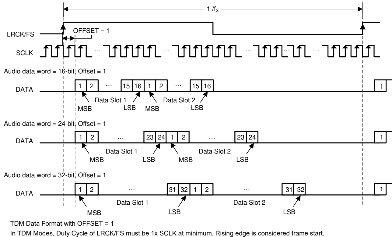
Figure 9-6. TDM 2 Audio Data Format
