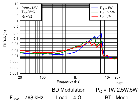
Figure 7-48. THD+N vs Frequency-BTL
