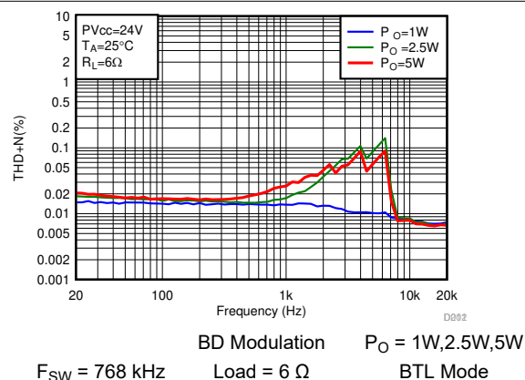
Figure 7-52. THD+N vs Frequency-BTL
