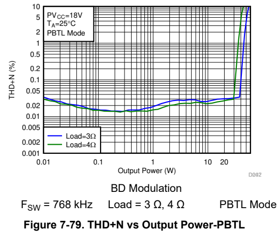
Figure 7-79. THD+N vs Output Power-PBTL
