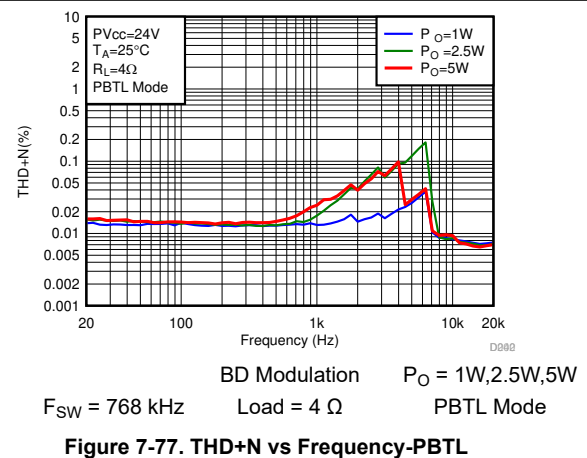
Figure 7-77. THD+N vs Frequency-PBTL
