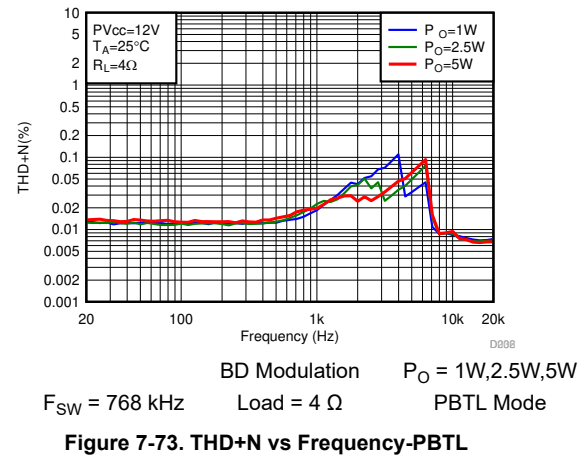
Figure 7-73. THD+N vs Frequency-PBTL
