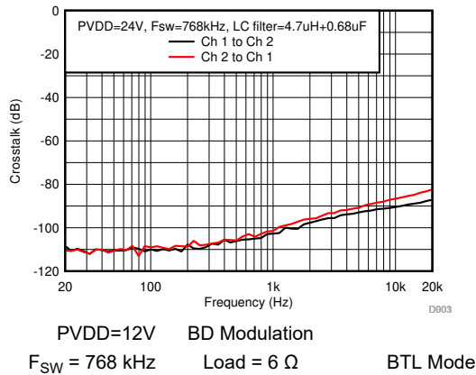
Figure 7-65. Crosstalk
