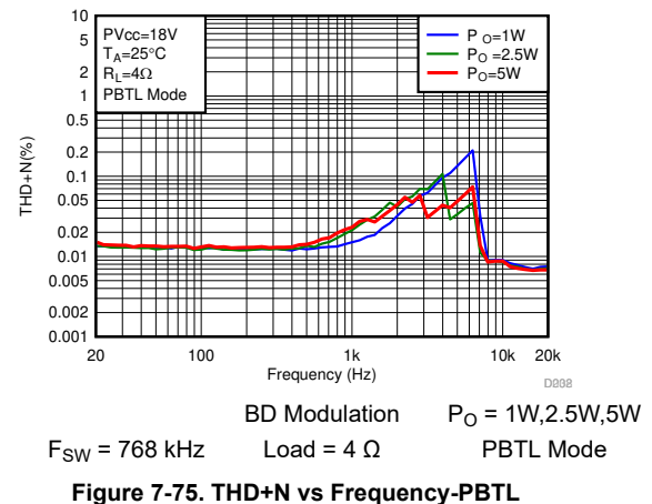
Figure 7-75. THD+N vs Frequency-PBTL
