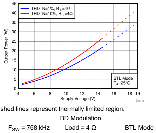
Figure 7-60. Output Power vs Supply Voltage
