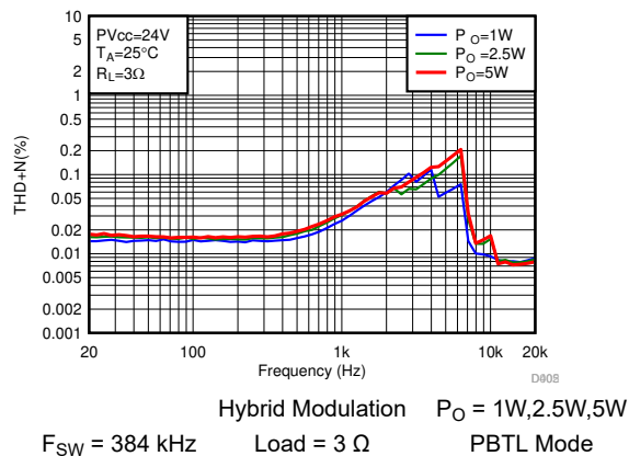
Figure 7-31. THD+N vs Frequency-PBTL
