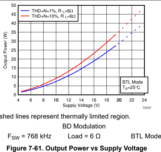
Figure 7-61. Output Power vs Supply Voltage
