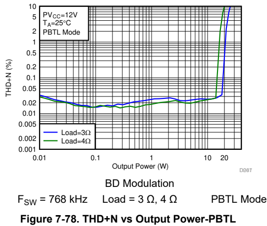
Figure 7-78. THD+N vs Output Power-PBTL
