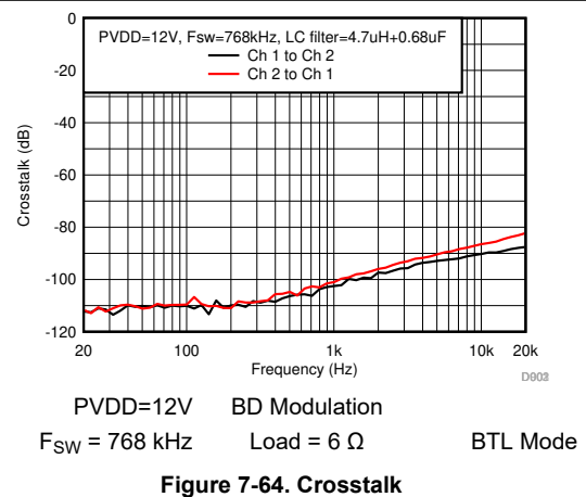
Figure 7-64. Crosstalk
