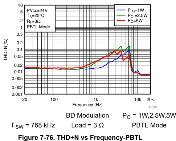
Figure 7-76. THD+N vs Frequency-PBTL
