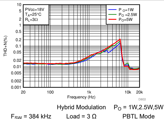
Figure 7-29. THD+N vs Frequency-PBTL
