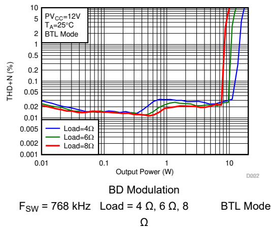
Figure 7-55. THD+N vs Output Power-BTL
