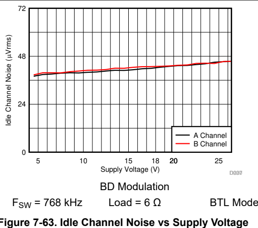
Figure 7-63. Idle Channel Noise vs Supply Voltage
