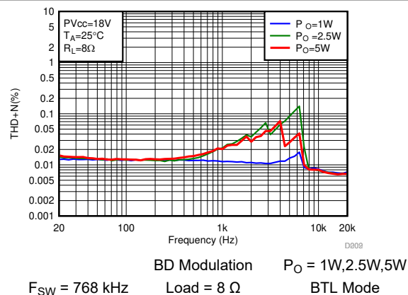
Figure 7-50. THD+N vs Frequency-BTL
