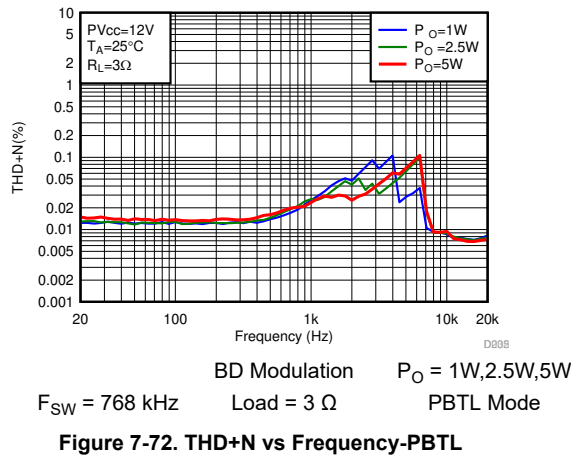
Figure 7-72. THD+N vs Frequency-PBTL
