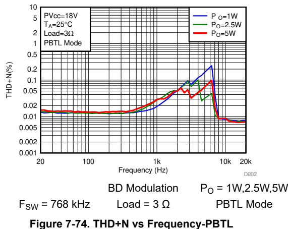
Figure 7-74. THD+N vs Frequency-PBTL
