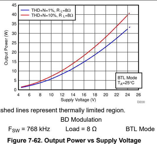
Figure 7-62. Output Power vs Supply Voltage
