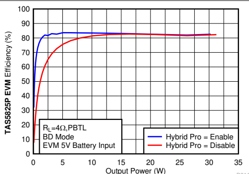
Figure 7-84. Efficiency vs Output Power
