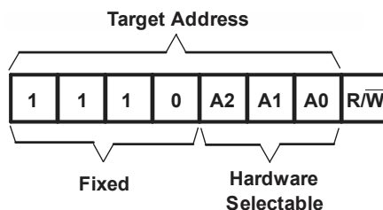
Figure 8-3. TCA9548A-Q1 Address
