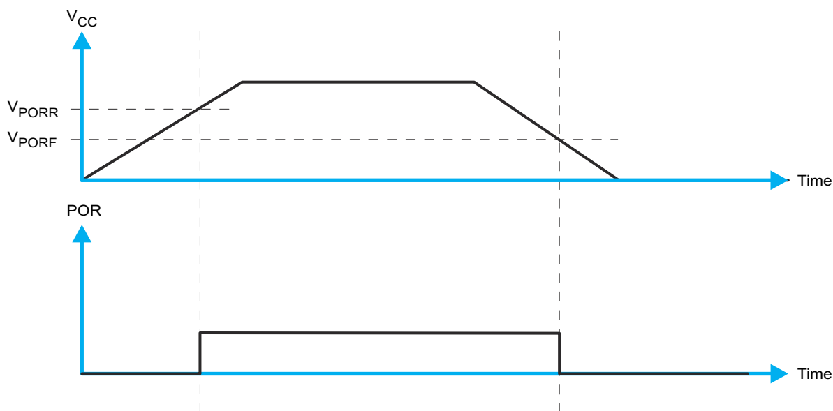
Figure 9-3. V_{POR} Example
