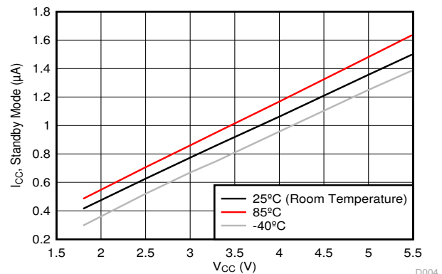
Figure 6-2. Standby Current ( I_{CC} ) vs Supply Voltage ( V_{CC} ) at three temperatures
