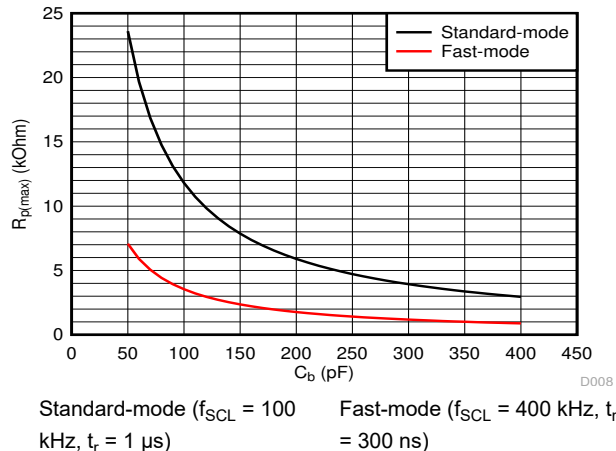
Figure 9-3. Maximum Pull-up Resistance ( R_{p(max)} ) vs Bus Capacitance ( C_b )
