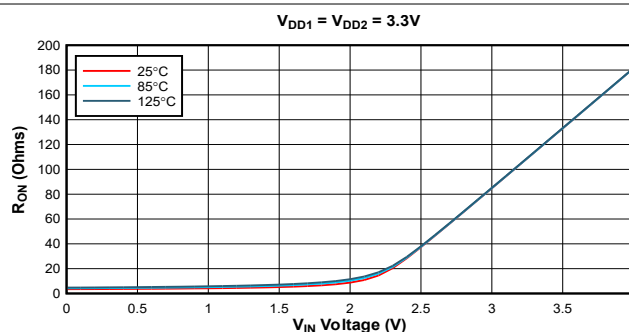
Figure 6-4. On-Resistance ( R_{ON} ) vs Input Voltage at Three Temperature Points
