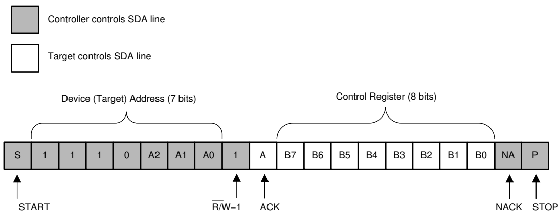
Figure 8-4. Read from Control Register
