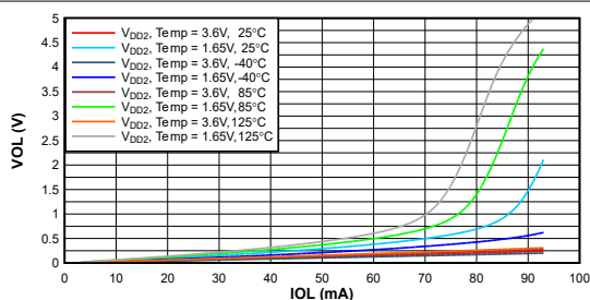
Figure 9-2. SDA Output Low Voltage ( V_{OL} ) vs Load Current ( I_{OL} ) at V_{DD2} Levels = 3.6V, 1.65V and T_A = -40^\circ\text{C} , 25^\circ\text{C} , 85^\circ\text{C} , 125^\circ\text{C}
