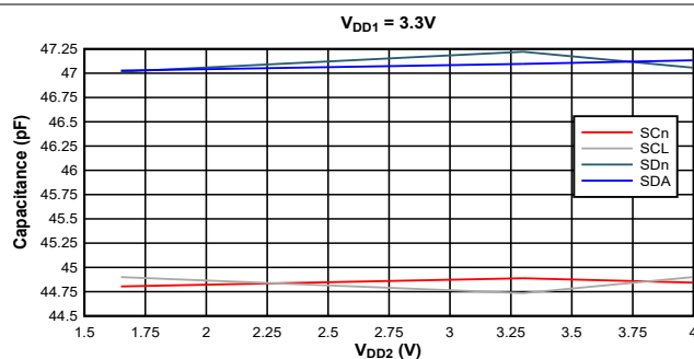
Figure 6-3. Target Channel (SCn/SDn) Capacitance ( C_{IO(OFF)} ) vs Supply Voltage ( V_{DD2} ) at 25°C
