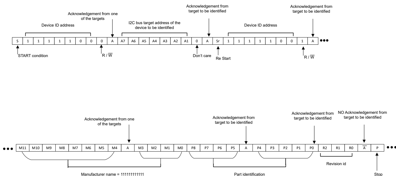
Figure 8-7. Device ID
