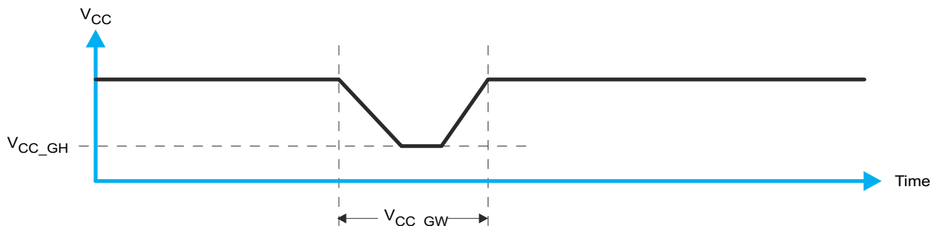
Figure 9-7. Glitch Width and Glitch Height
