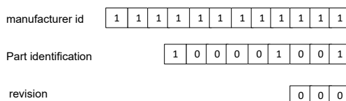
Figure 8-7. Device ID
