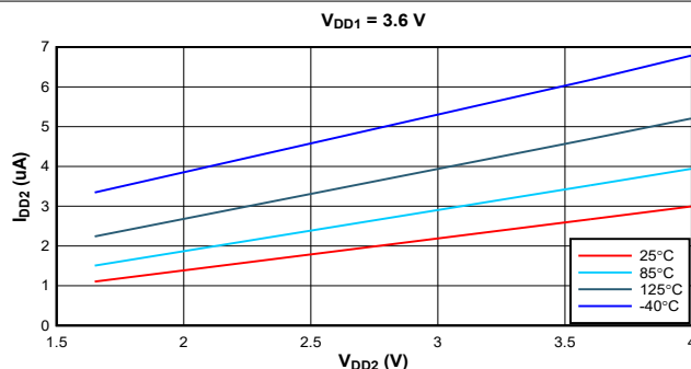
Figure 9-3. Standby Current ( I_{DD} ) vs Supply Voltage ( V_{DD2} ) at Four Temperature Points
