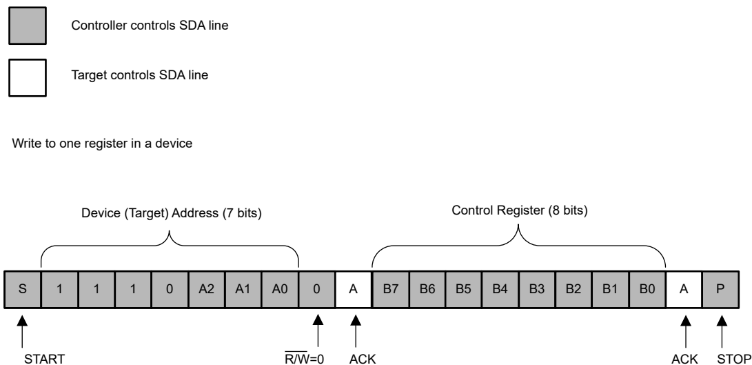
Figure 8-3. Write to Register
