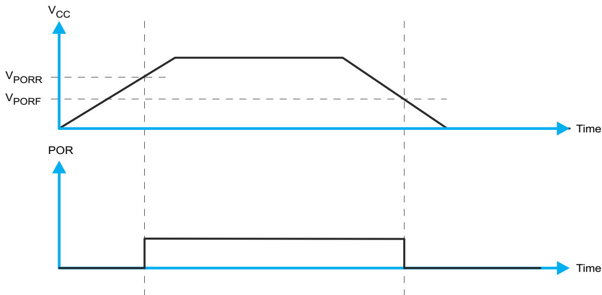
Figure 9-8. V_{POR}
