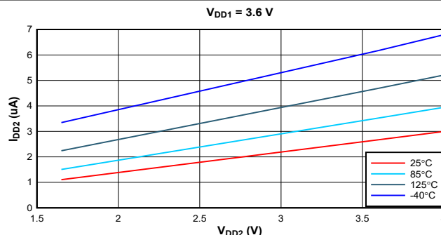
Figure 6-2. Standby Current ( I_{DD} ) vs Supply Voltage ( V_{DD2} ) at Four Temperature Points
