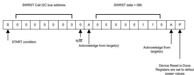
Figure 8-6. Software Reset Sequence
