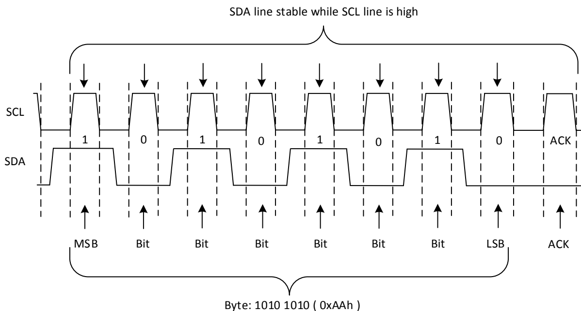
Figure 8-2. Bit Transfer
