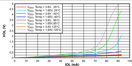
Figure 6-1. SDA Output Low Voltage ( V_{OL} ) vs Load Current ( I_{OL} ) at V_{DD2} Levels = 3.6V, 1.65V and T_A = -40°C, 25°C, 85°C, 125°C
