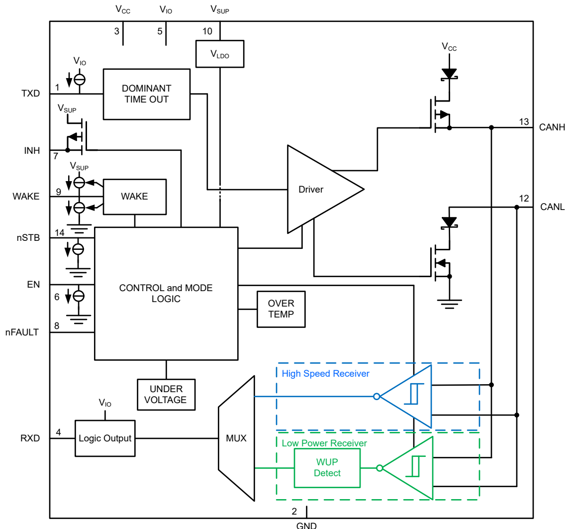
Figure 7-1. TCAN1043A-Q1 Functional Block Diagram
