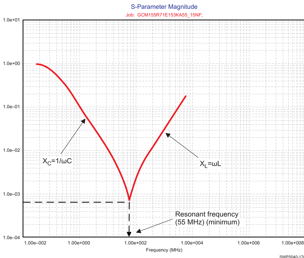
Figure 7-14. Typical Impedance Profile of a Capacitor
